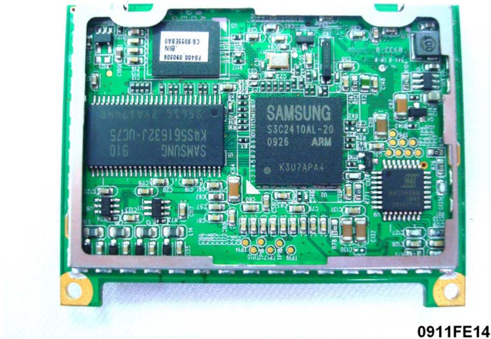
(28) EUT Photo
