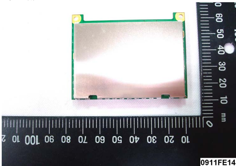
(26) EUT Photo
