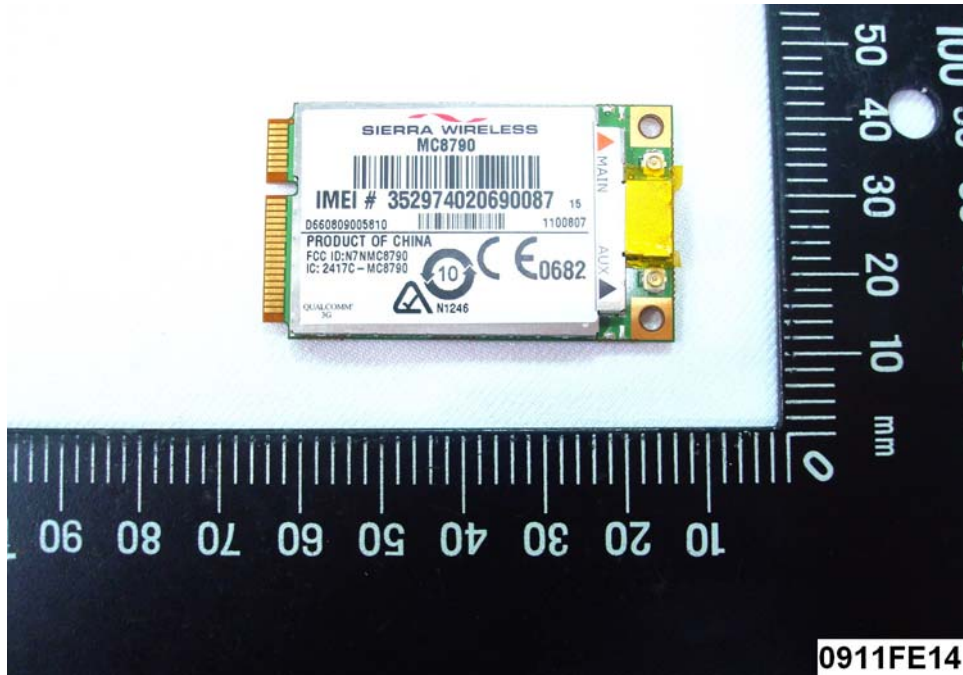
(7) EUT Photo
