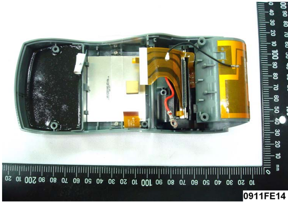
(29) EUT Photo
