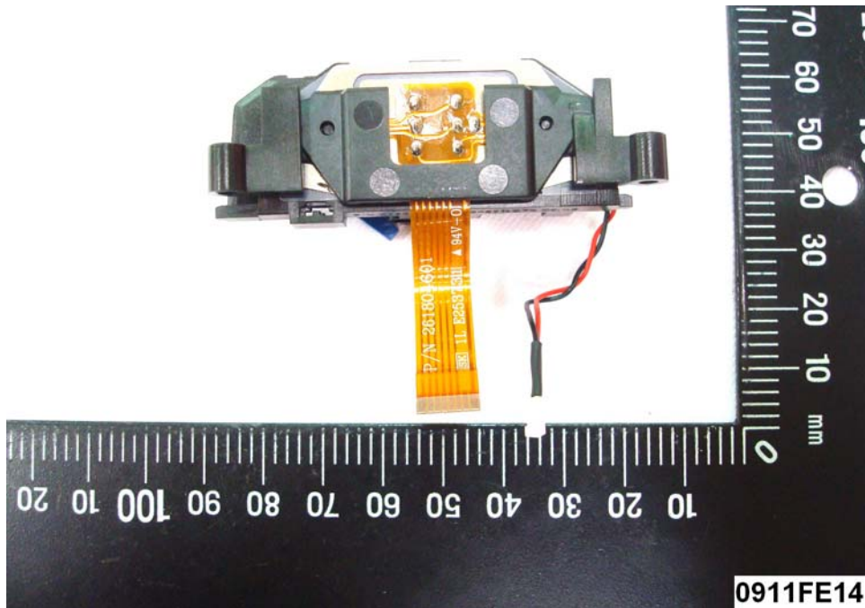
(23) EUT Photo
