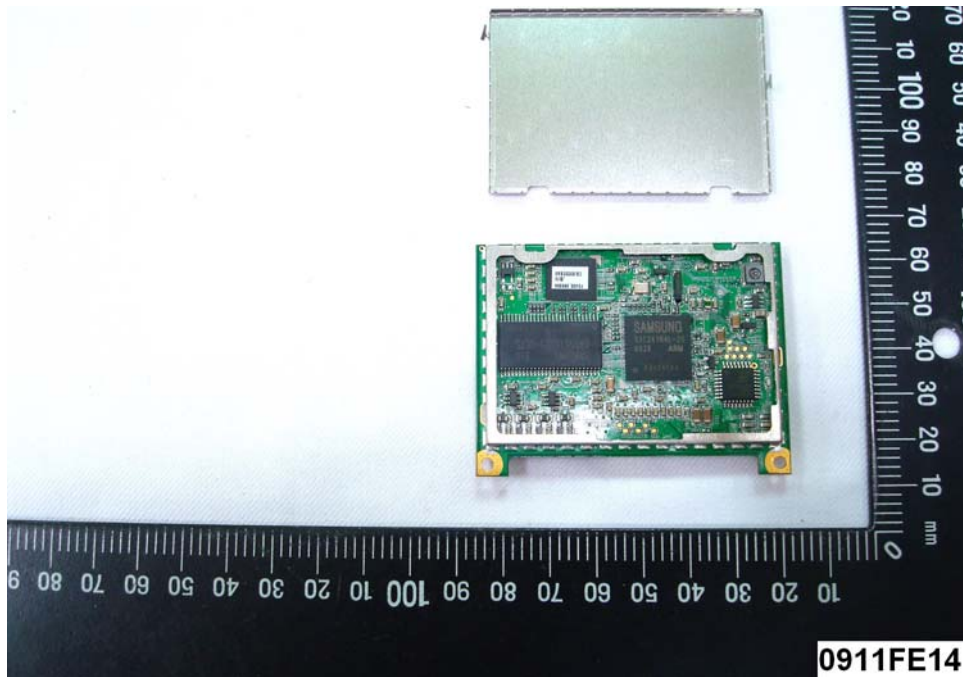
(27) EUT Photo
