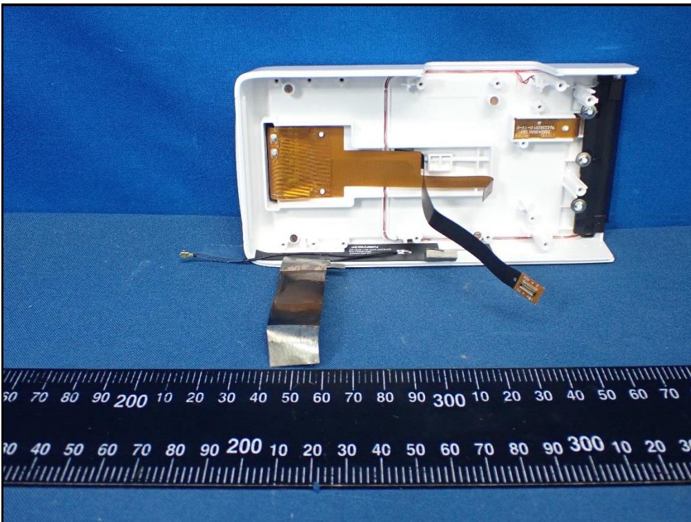
Antenna- WWAN-Aux
