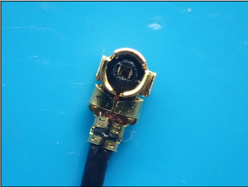
Antenna- WWAN-Aux
