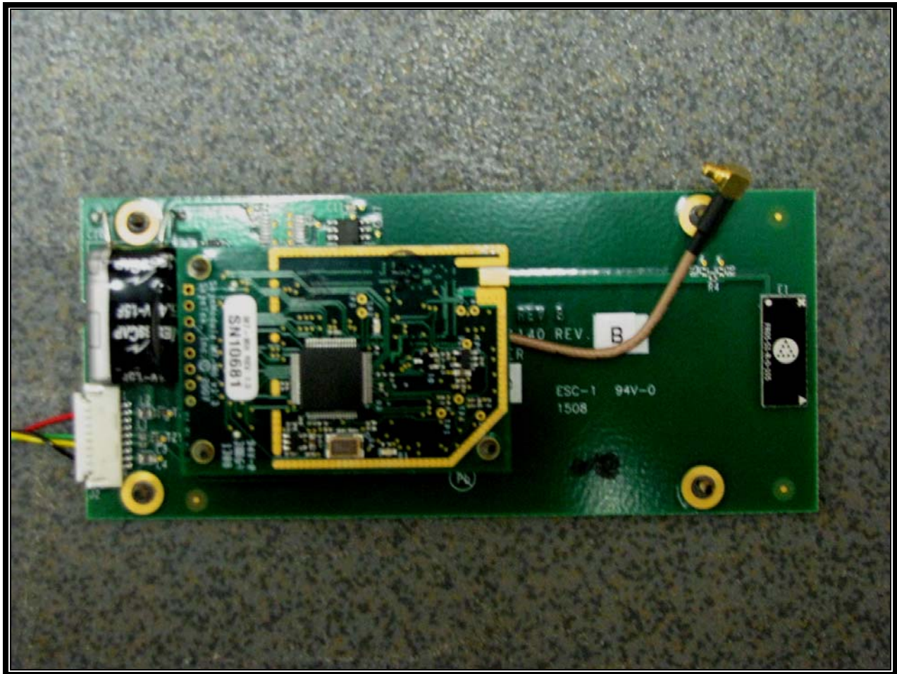
Photograph 4: Top of Main PCB with RFID PCB Installed
