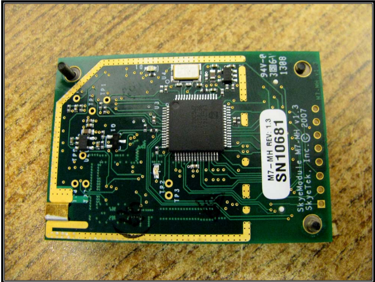
Photograph 8: Bottom of RFID PCB
