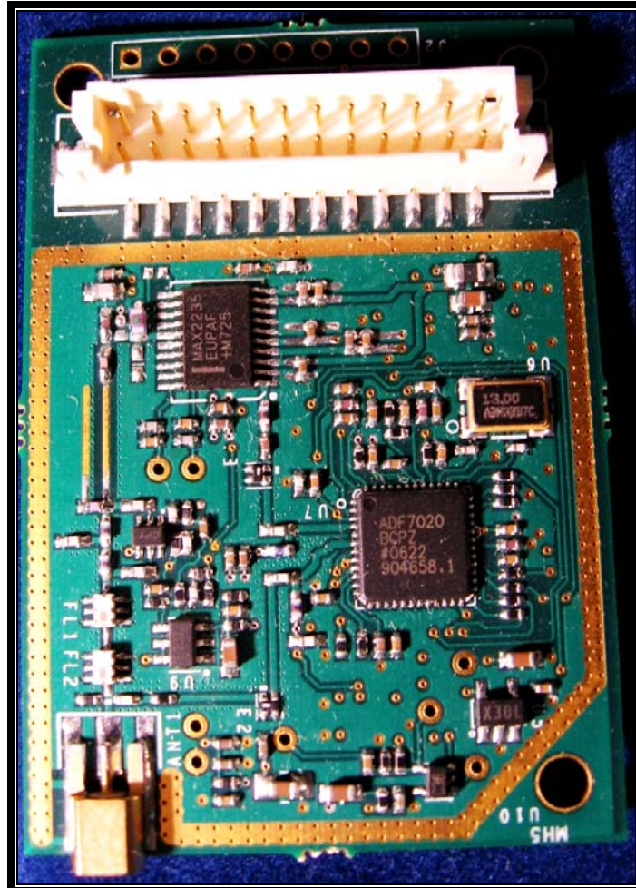
Photograph 7: Top of RFID PCB without Shield
