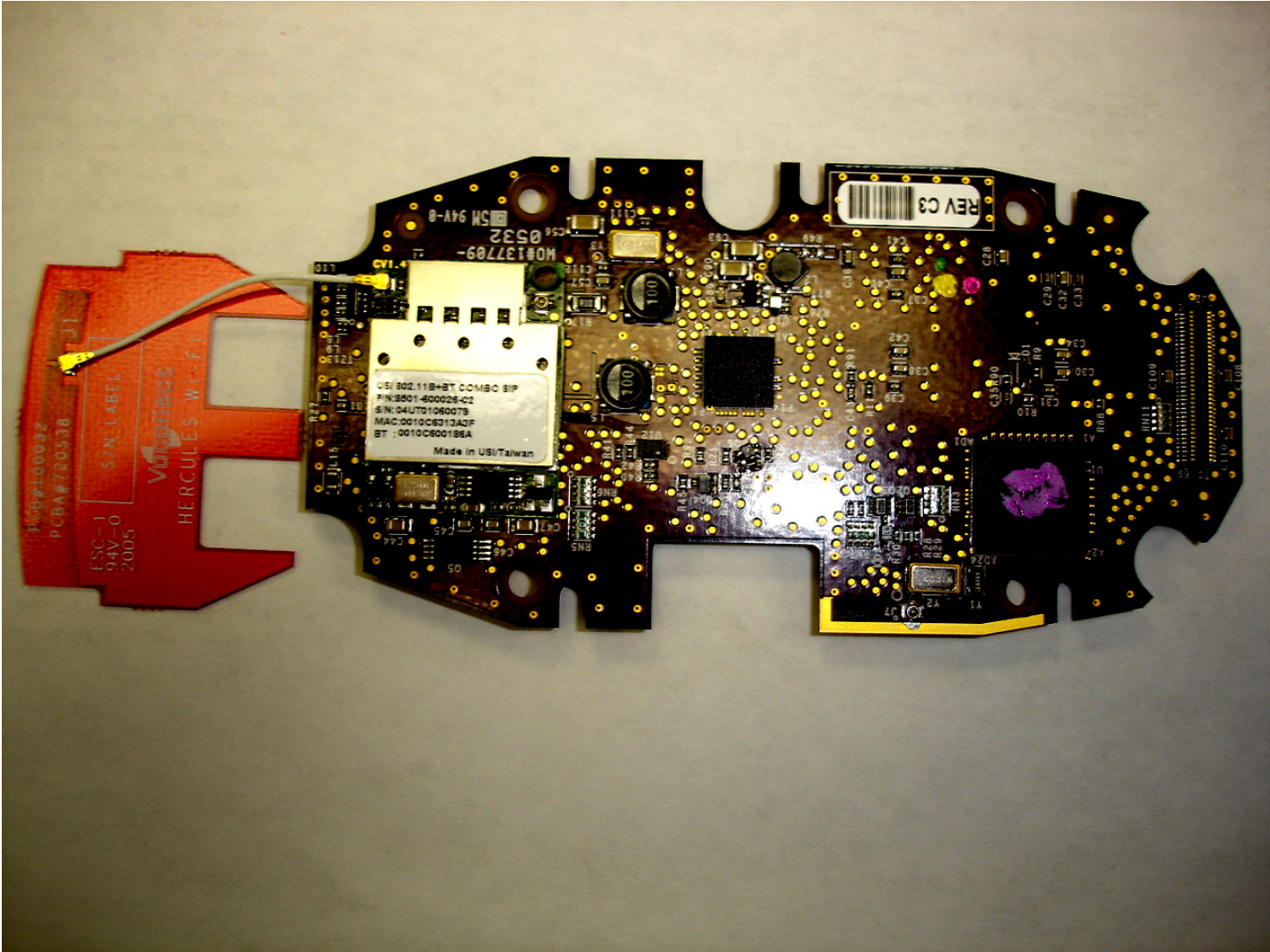
Talkman T5 PWB Board Bottom View
