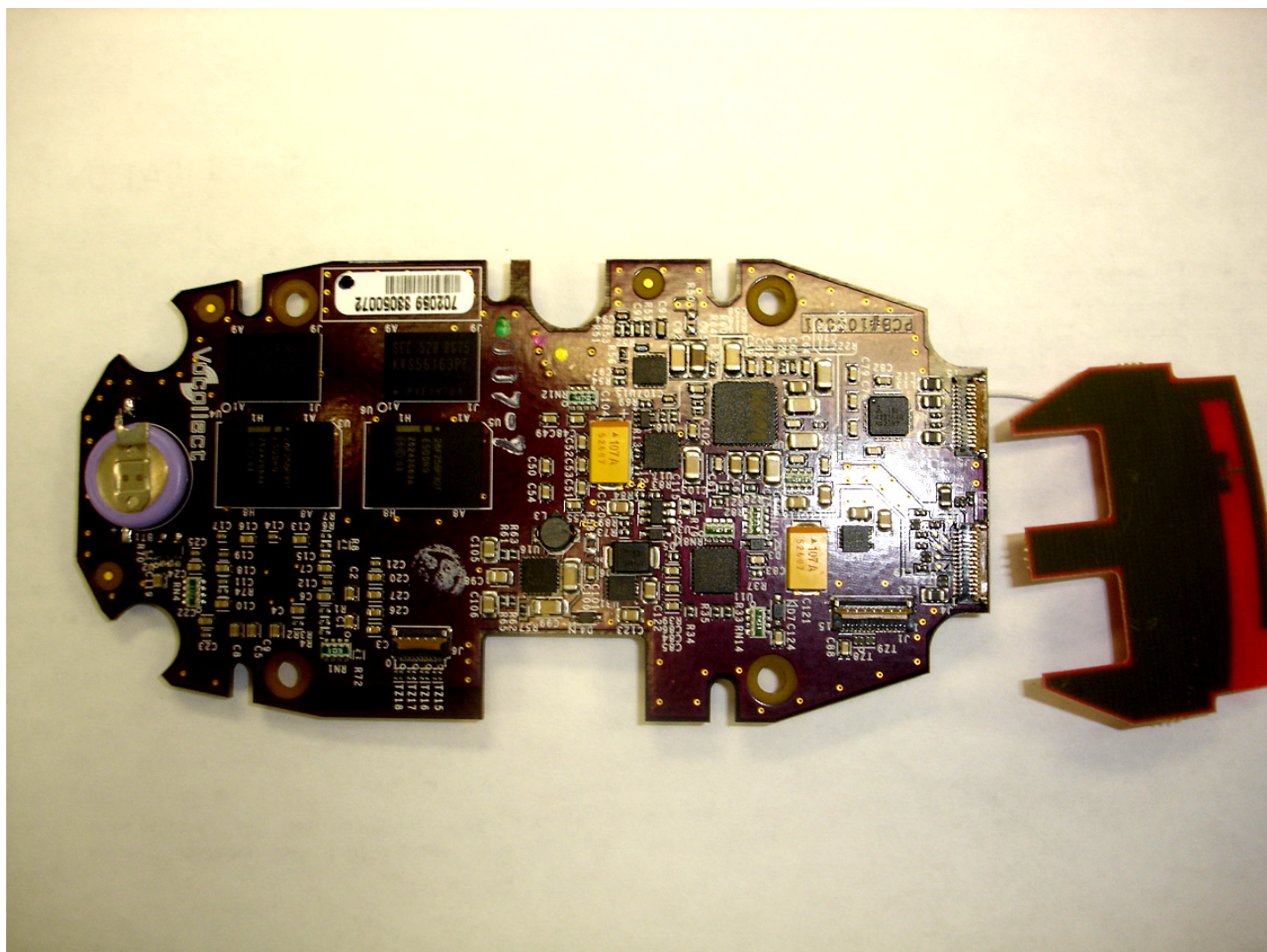
Talkman T5 PWB Board Top View
