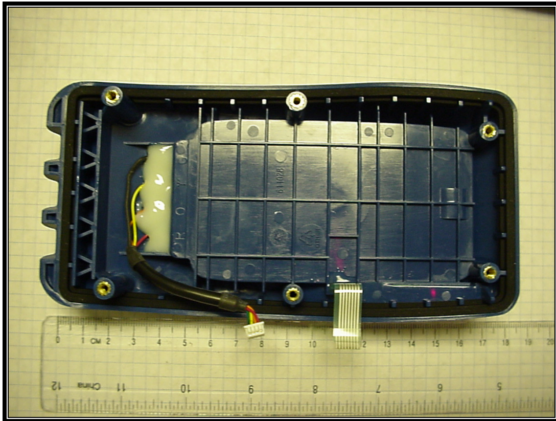
Photograph 10: Inside Top
