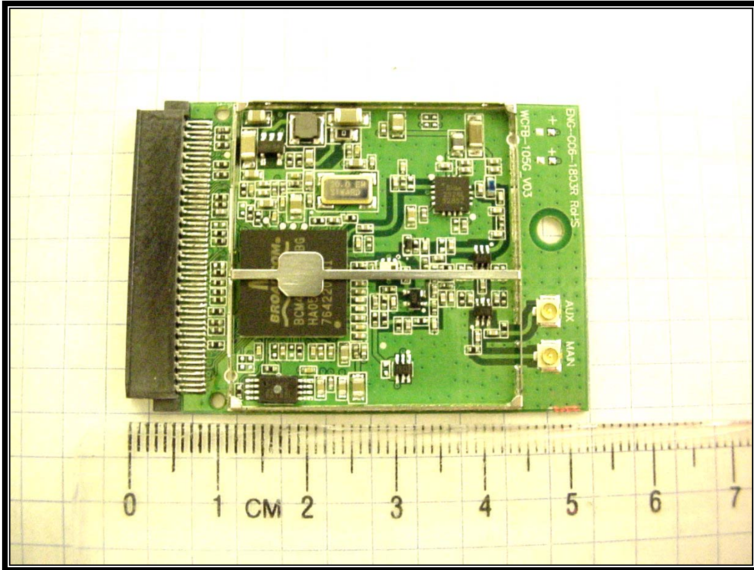
Photograph 19: Radio PCB Top with Shield Removed
