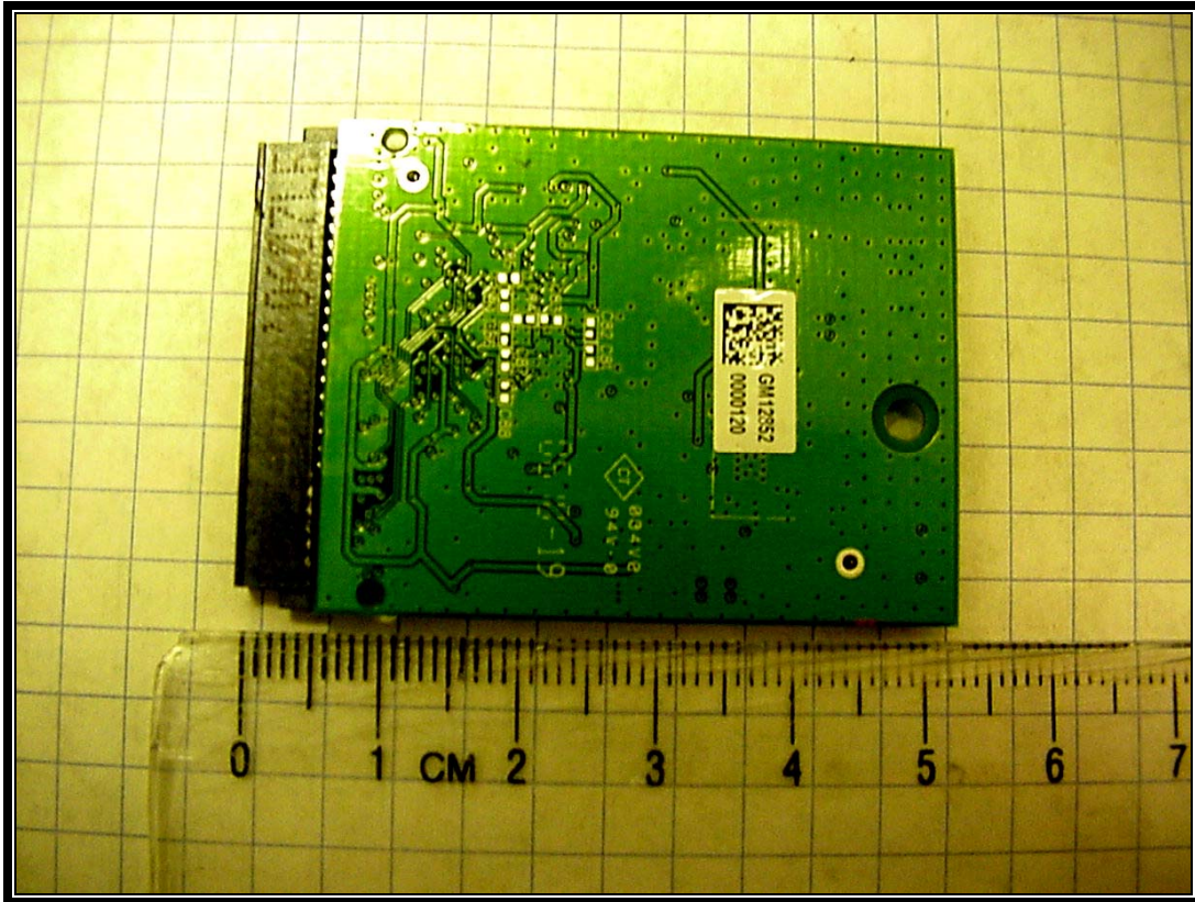
Photograph 20: Radio PCB Bottom View
