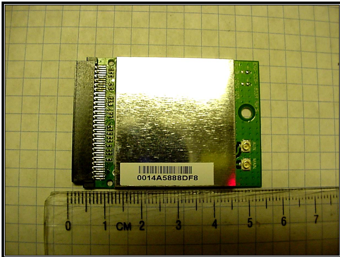
Photograph 18: Radio PCB Top with Shield
