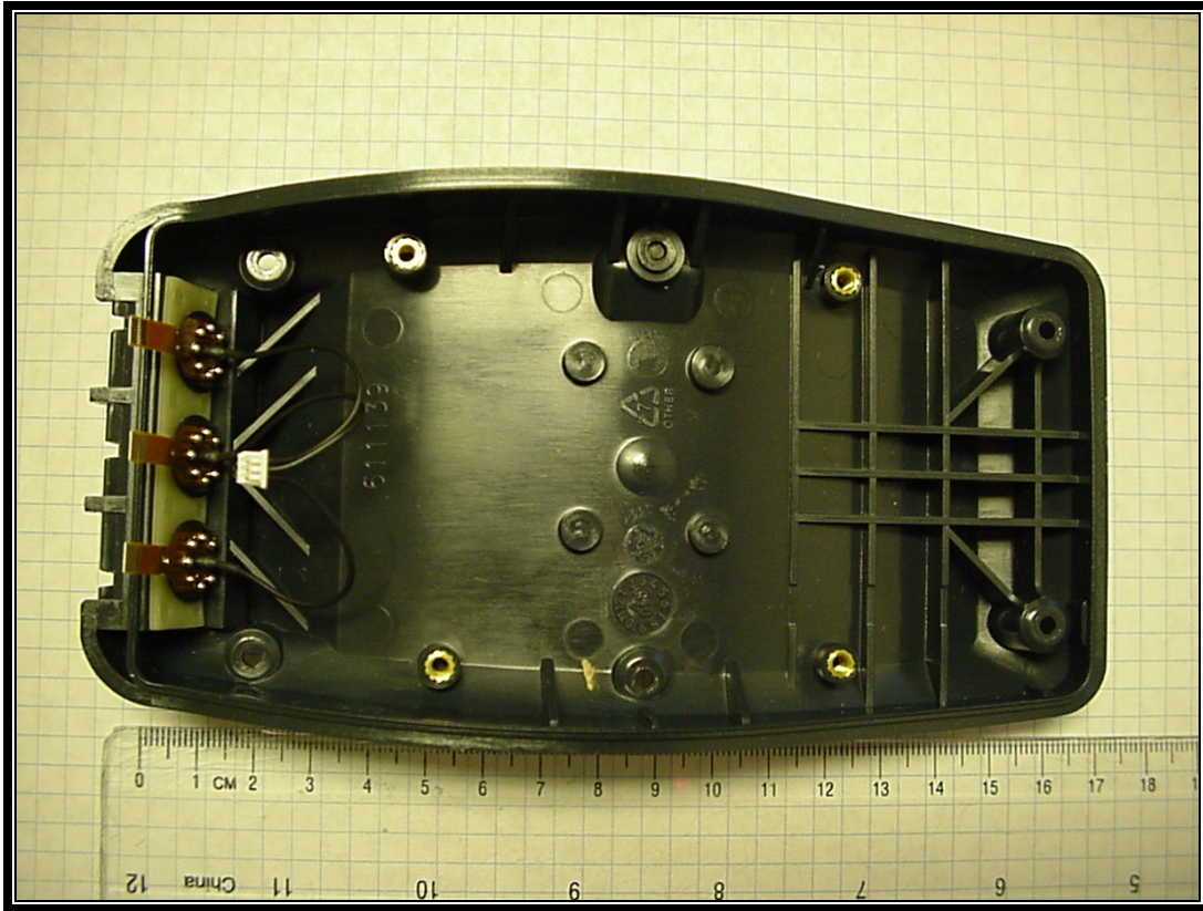
Photograph 11: Inside Bottom
