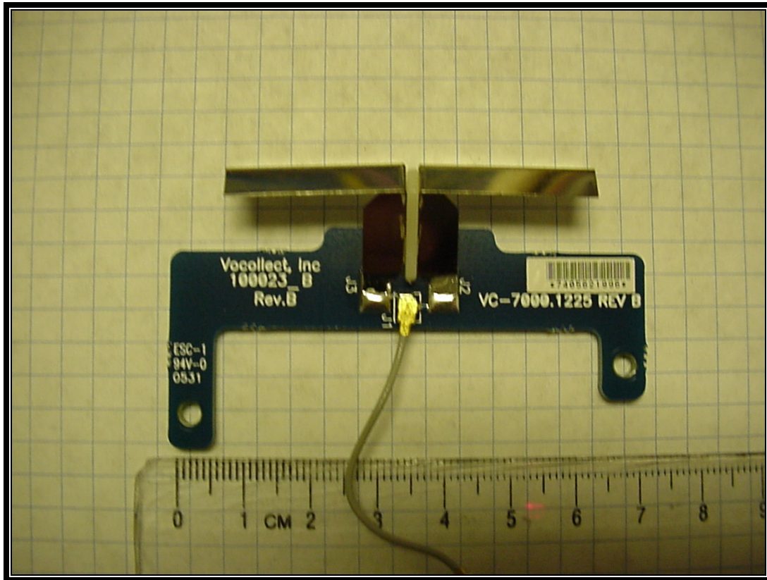
Photograph 14: Top of Antenna
