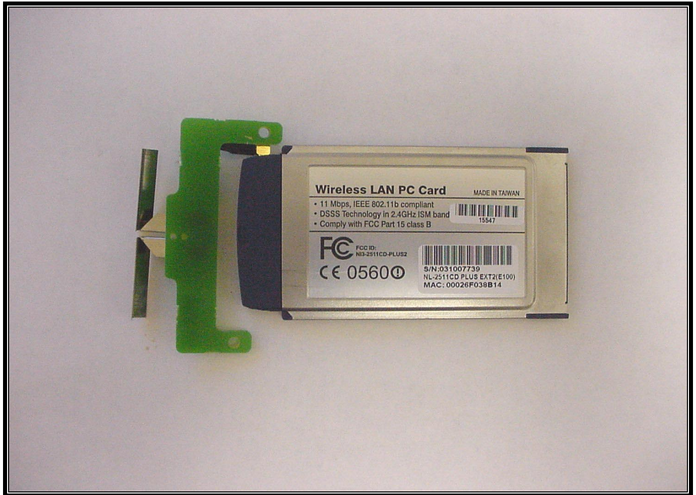
PHOTOGRAPH 17: WLAN CARD REAR WITH ANTENNA
