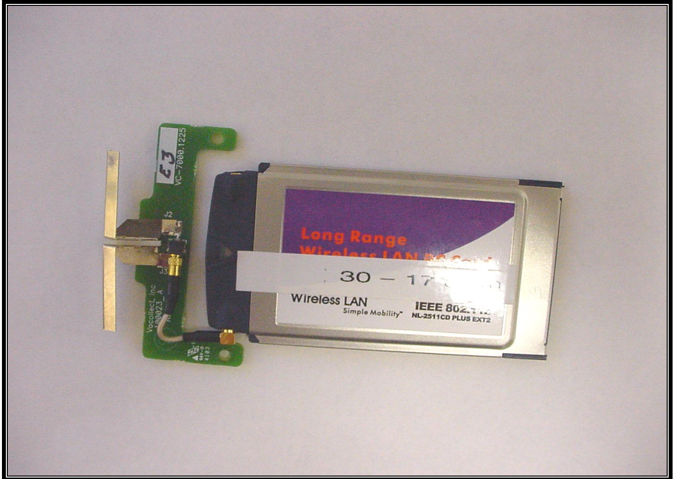
PHOTOGRAPH 16: WLAN CARD FRONT WITH ANTENNA
