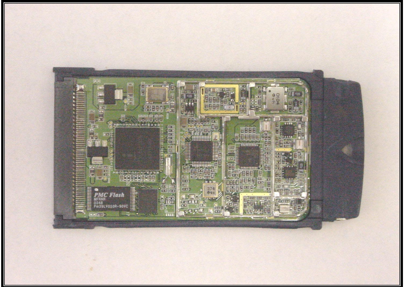
PHOTOGRAPH 23: TOP VIEW WLAN WITHOUT SHIELD
