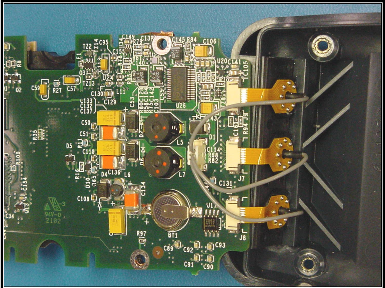
PHOTOGRAPH 21: PCB CONNECTIONS
