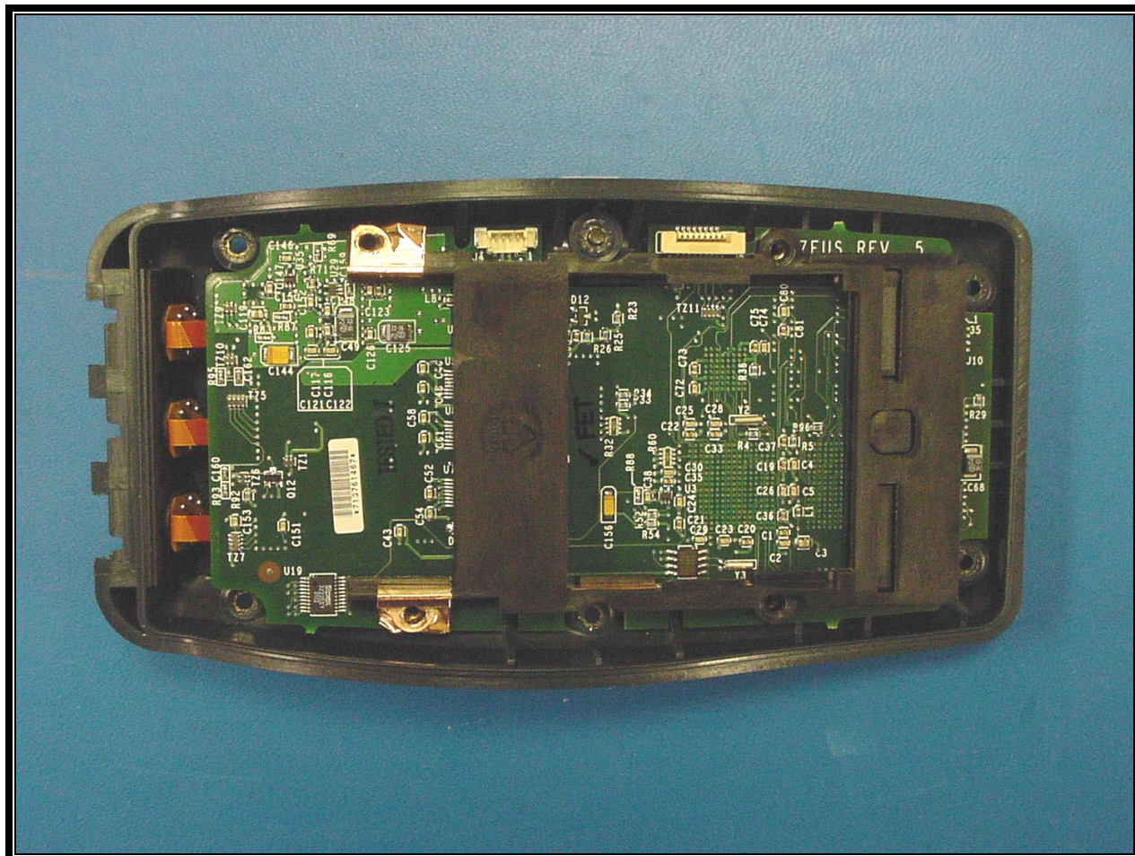
PHOTOGRAPH 13: PCB TOP
