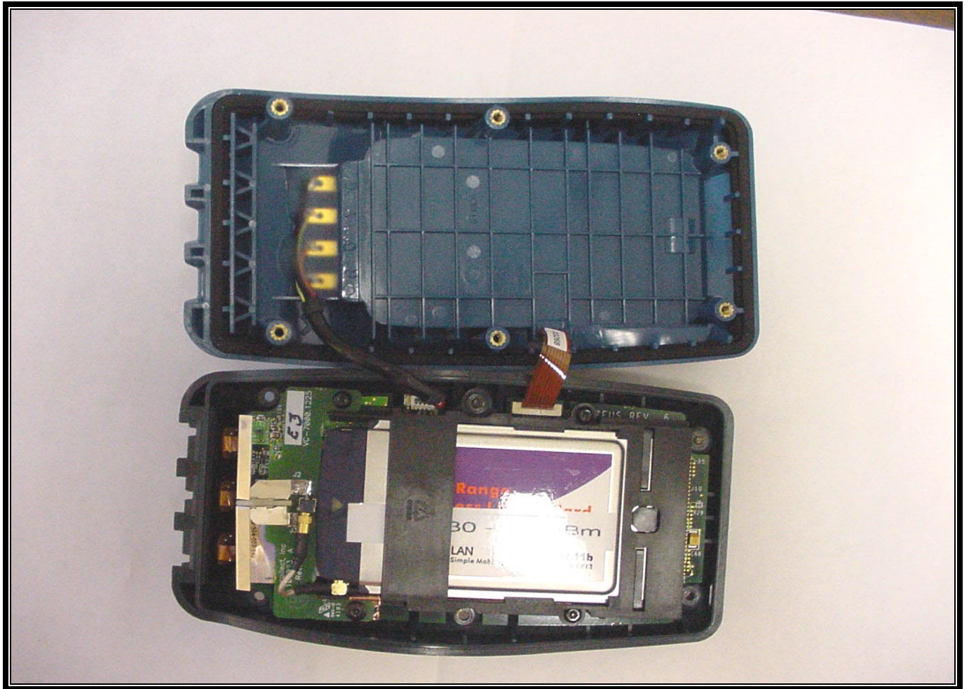
PHOTOGRAPH 9: OVERALL INTERNAL VIEW
