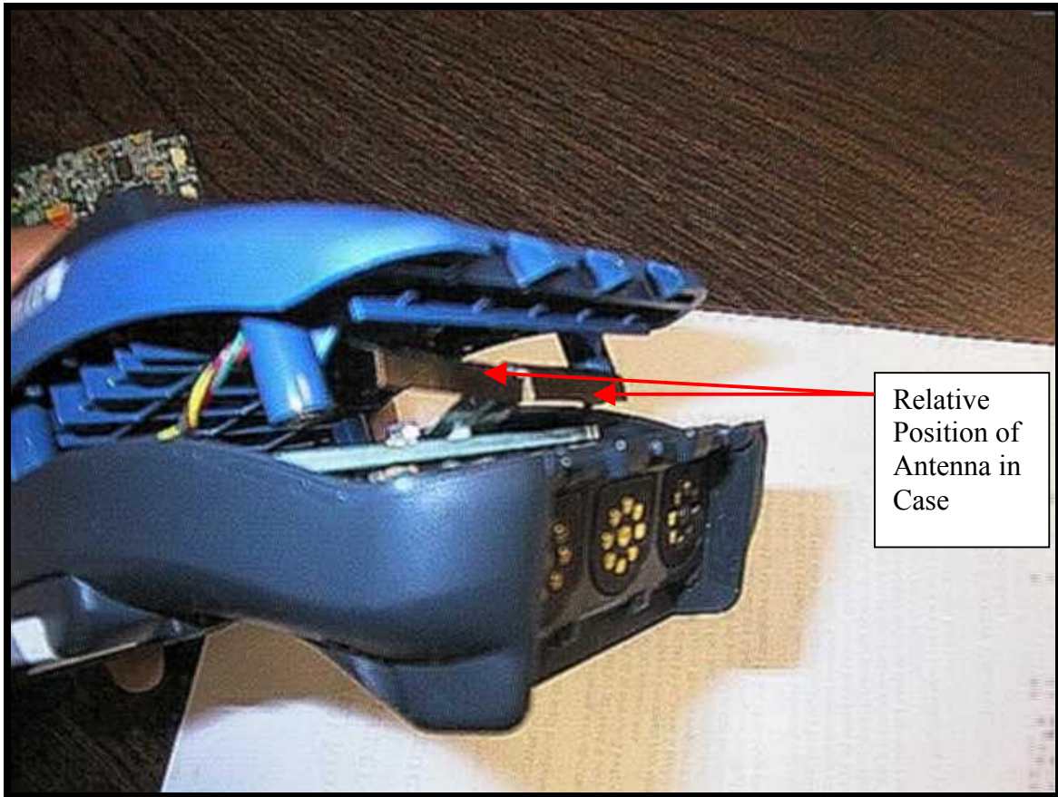
Relative Position of Antenna Within the Case
