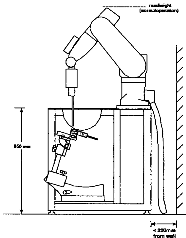
DASY3 Compact Version – Side View
