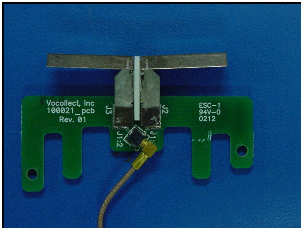
PHOTOGRAPH 18: ANTENNA FRONT
