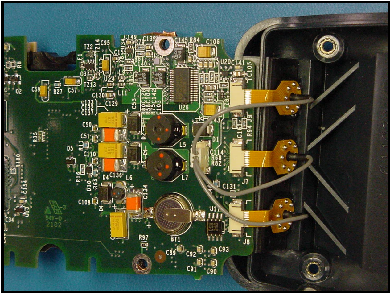
PHOTOGRAPH 20: PCB CONNECTIONS
