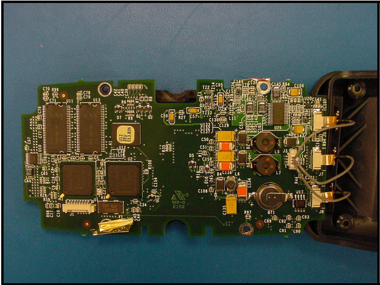
PHOTOGRAPH 15: PCB REAR WITHOUT SHIELD
