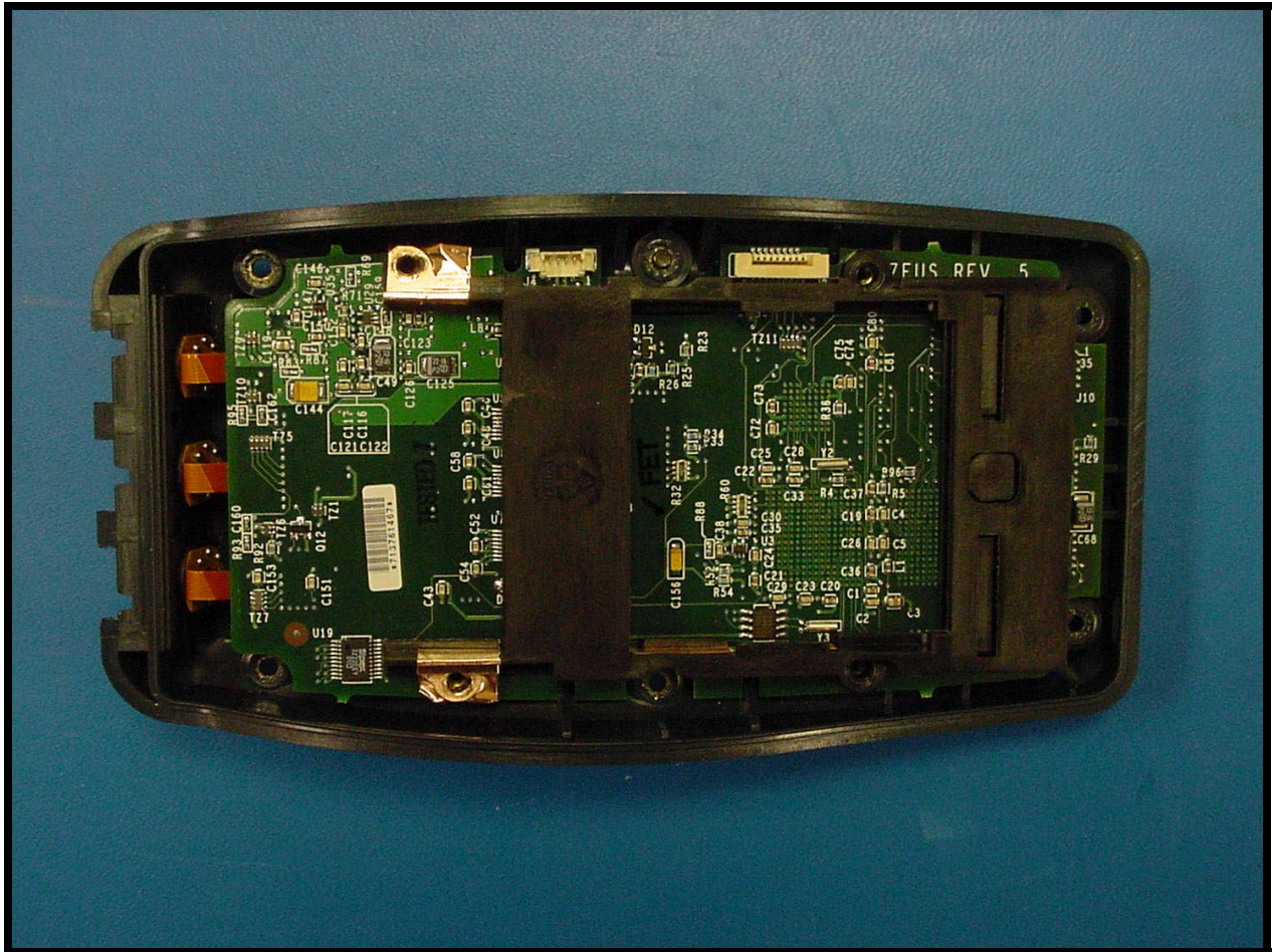
PHOTOGRAPH 13: PCB TOP
