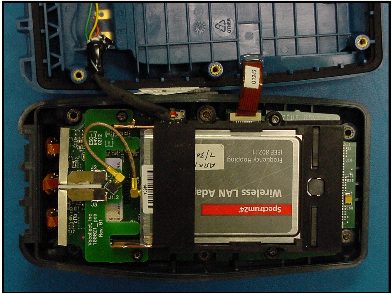
PHOTOGRAPH 10: INTERNAL VIEW WITH WLAN ADAPTER
