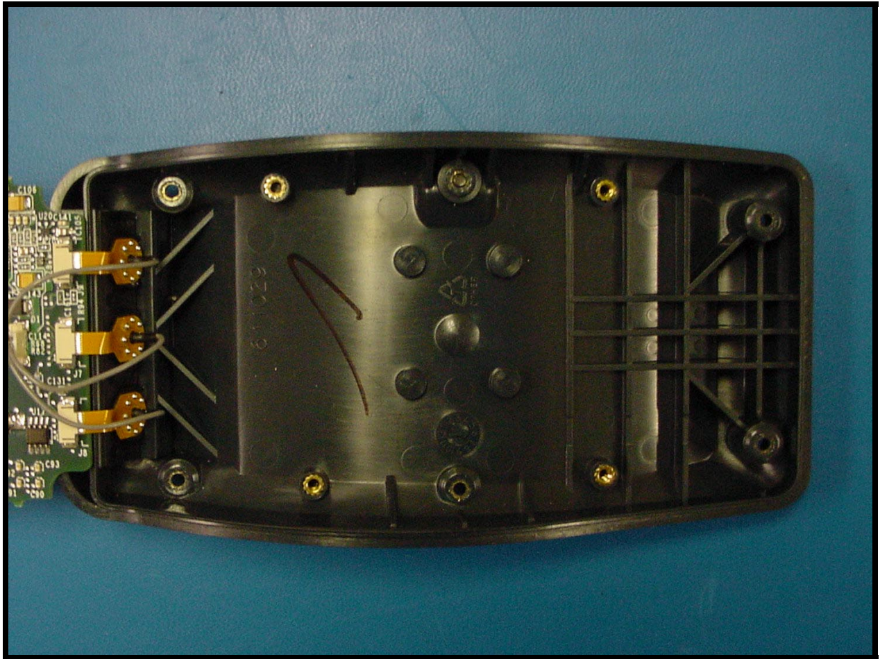
PHOTOGRAPH 12: INSIDE REAR COVER
