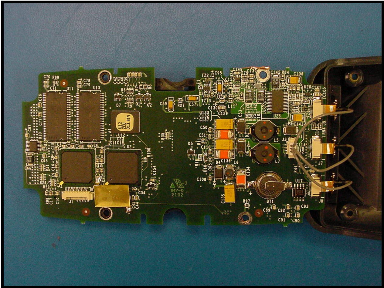
PHOTOGRAPH 14: PCB REAR WITH SHIELD
