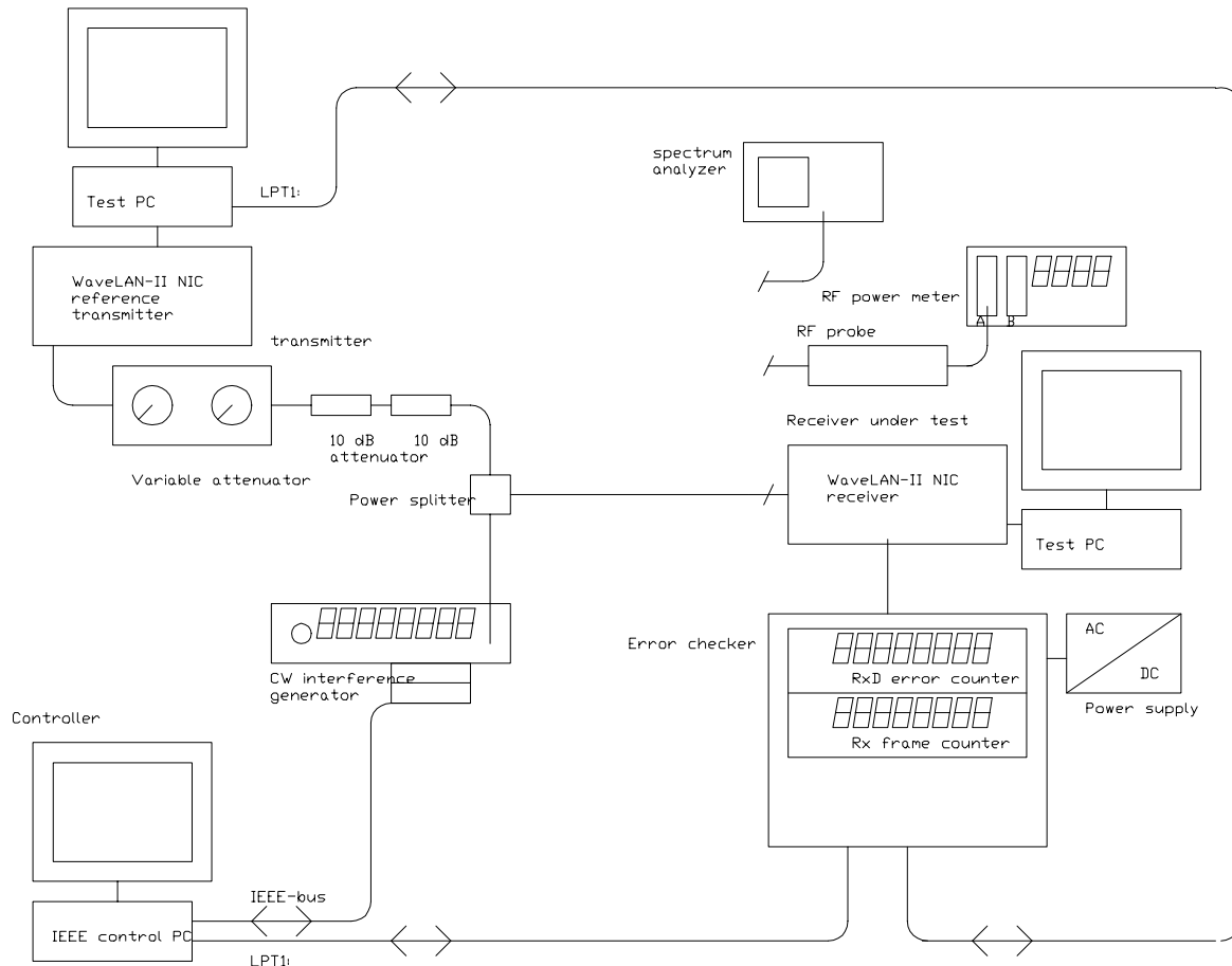
Figure 1, measurement test set-up.
