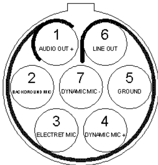
Apollo Headset Connector Yellow, Single Key Viewed from back / solder side
