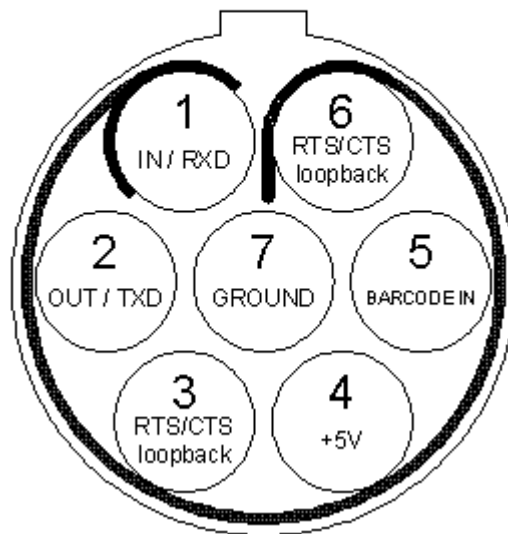
Apollo Serial Connector, Conn 2 Blue, Double Key (60 degrees) Viewed from back / crimp side
