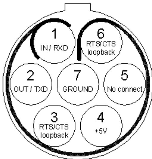
Apollo Serial Connector, Com 1 Red, Double Key (30 degrees) Viewed from back / crimp side
