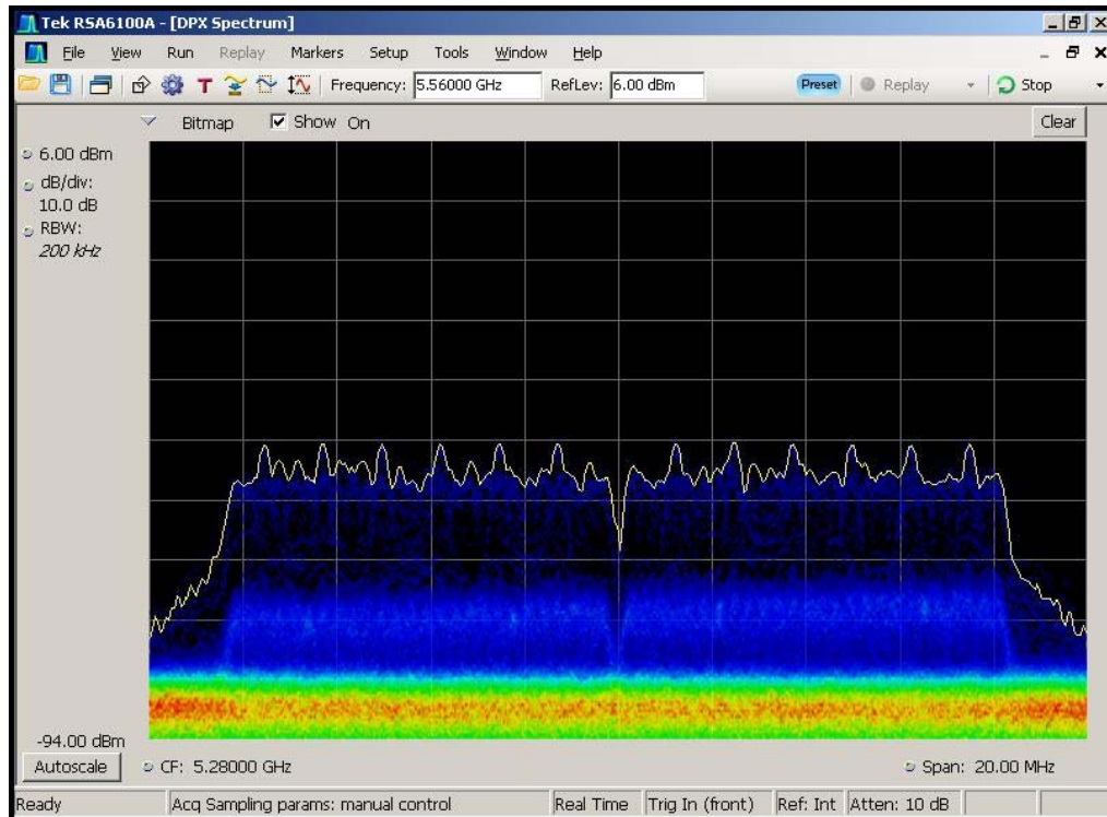
Figure 6-3. Real-Time Spectrum Display, WLAN Traffic (Streaming Video)
