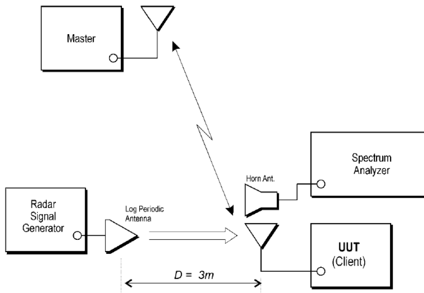
Figure 3-1. Radiated Test Setup for DFS
