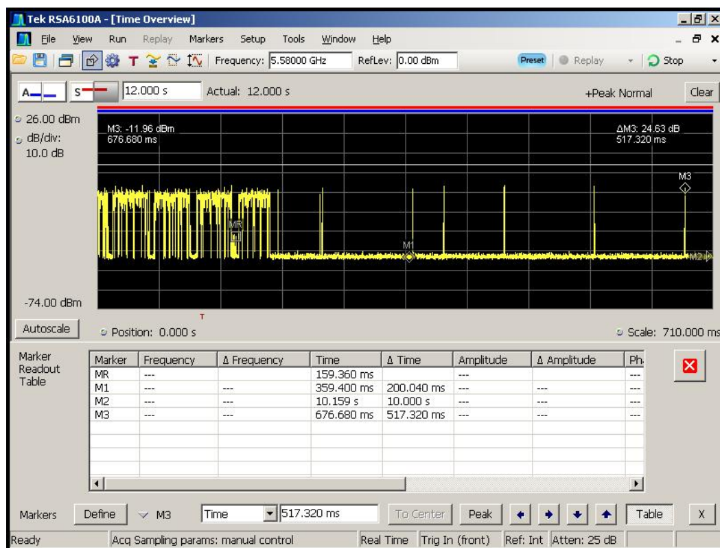
Figure 6-5. Aggregate Time Plot
