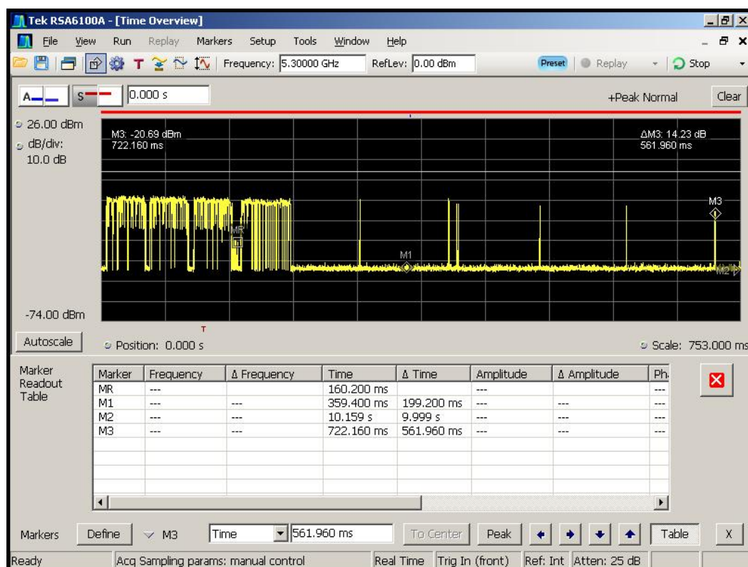
Figure 5-5. Aggregate Time Plot
