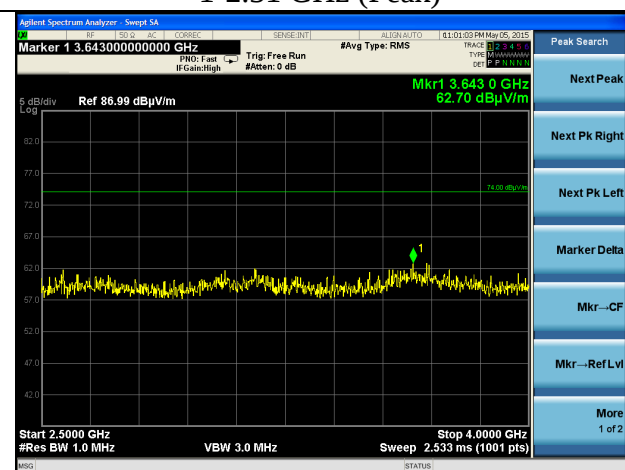
2.5-4 GHz (Peak)
