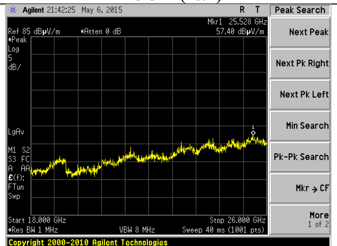
18-26 GHz (Peak)
