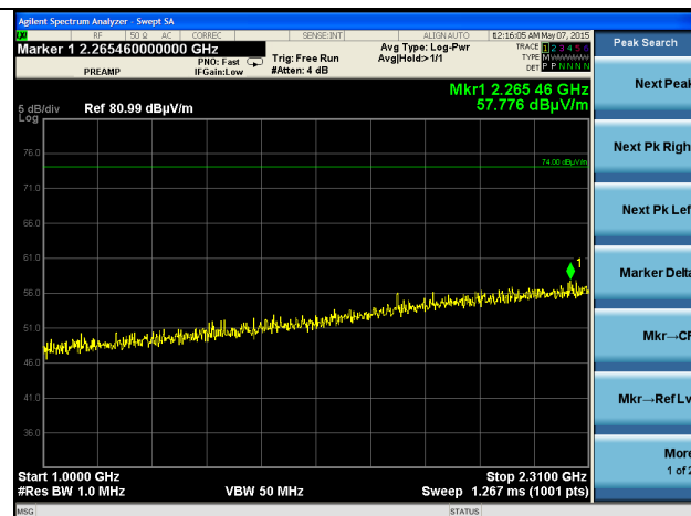
1-2.31 GHz (Peak)
