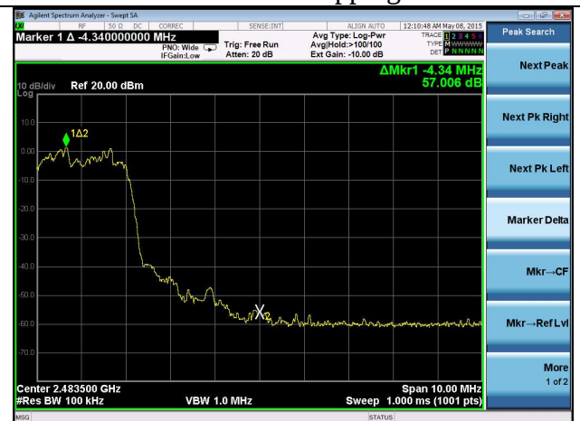
EDR-3 – Hopping
