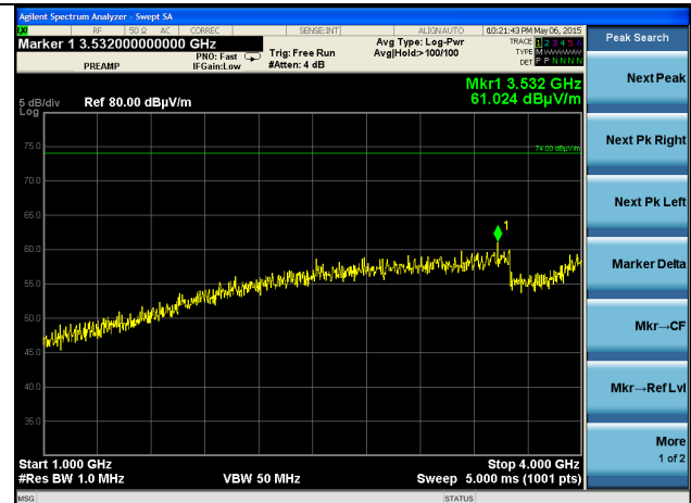
1-4 GHz (Peak)
