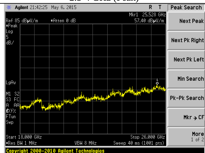
18-26 GHz (Peak)
