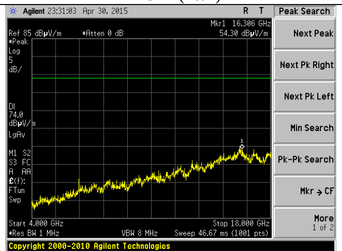
4-18 GHz (Peak)
