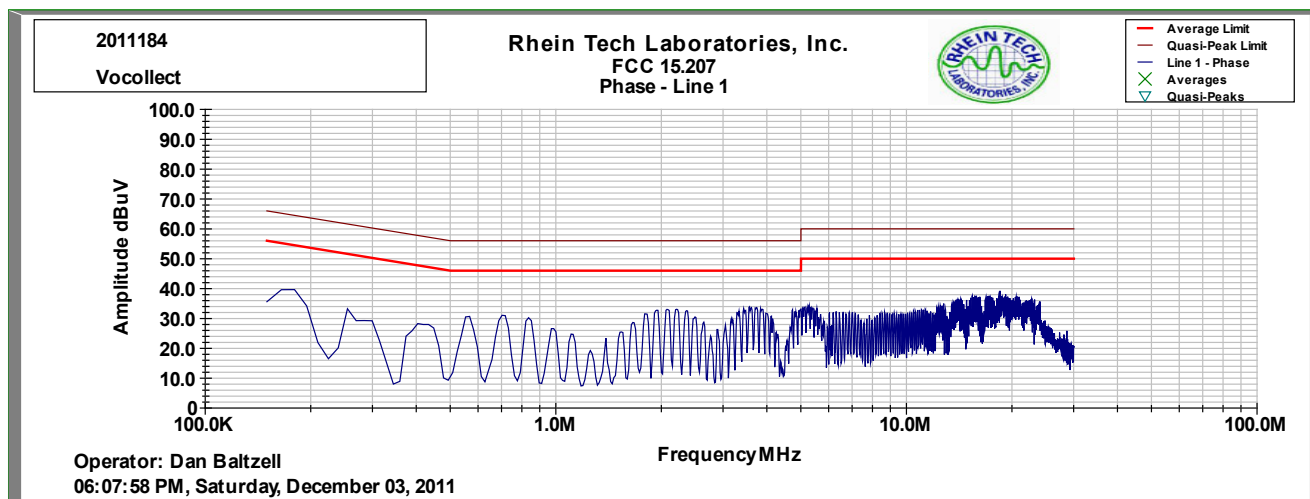
Plot 9-4: Conducted Emissions Receive Channel 6 FHSS/DSSS Hot Side
