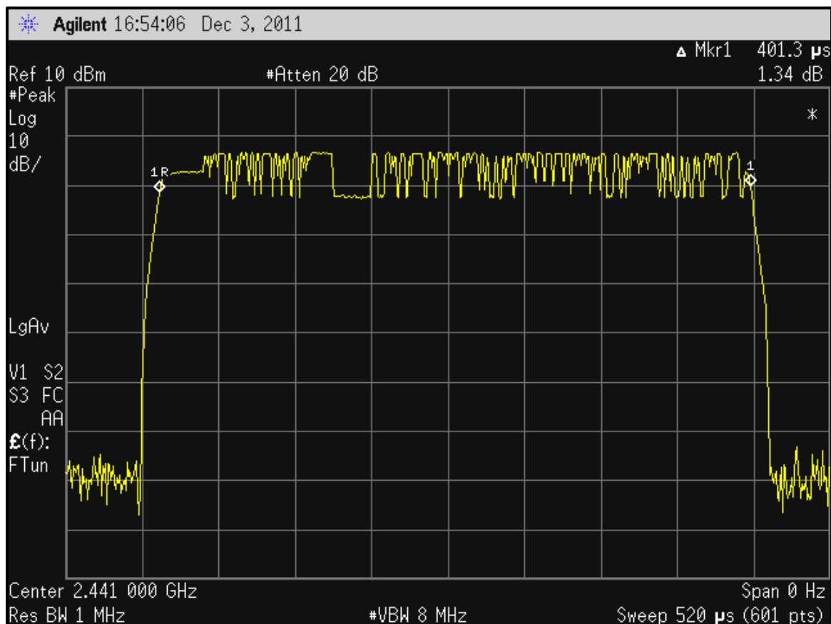
Plot 8-2: Time of Occupancy (Dwell Time)
