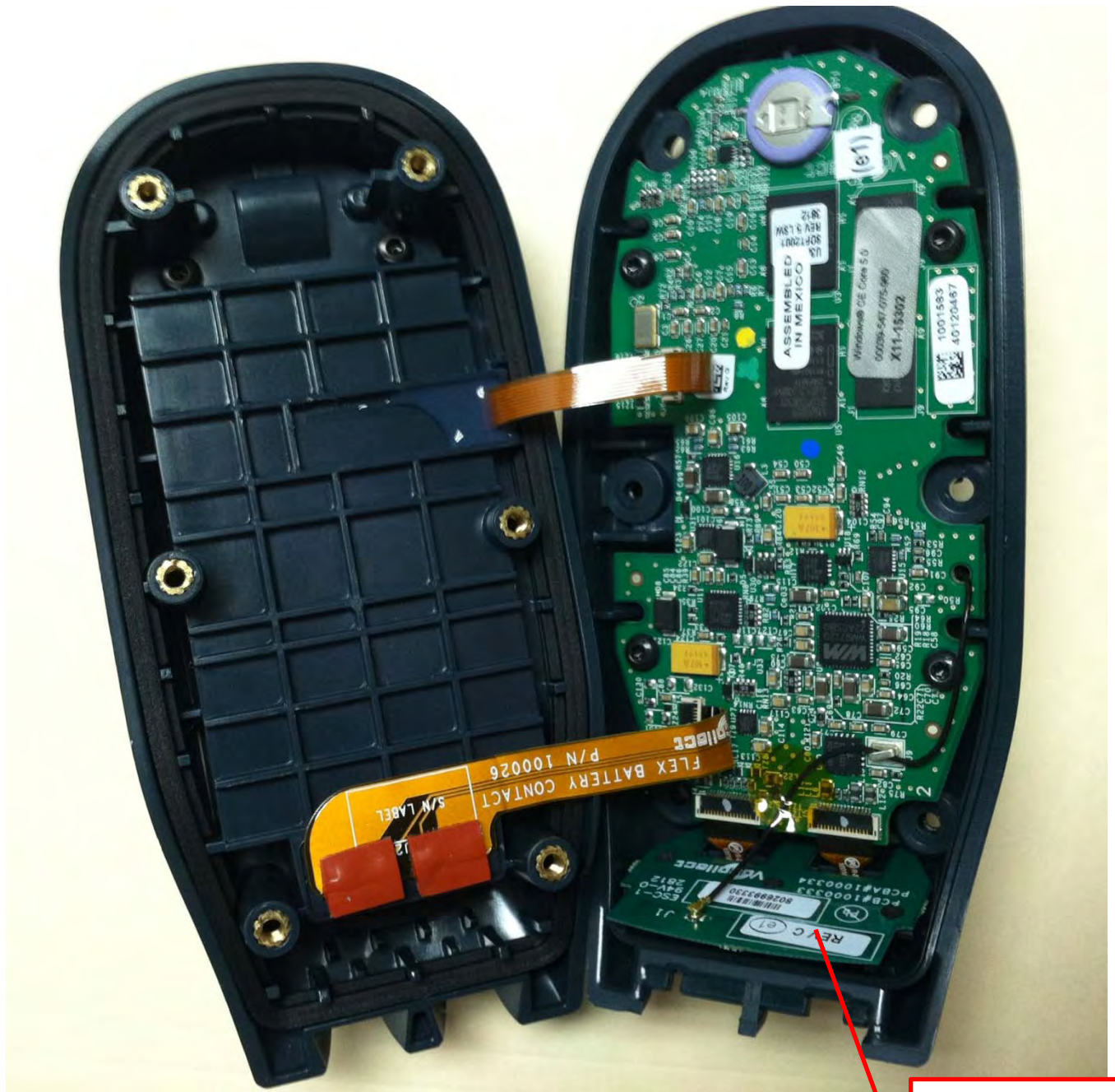
WiFi Antenna
