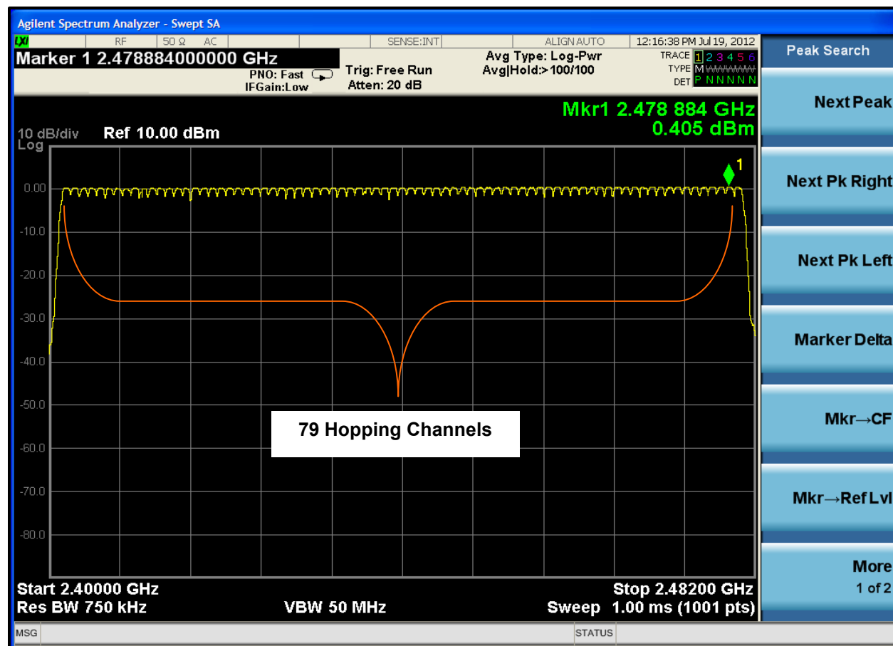
Plot 8-1: Number of Hopping Frequencies
