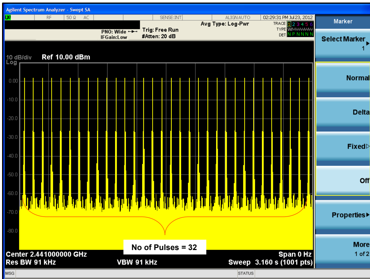
Plot 8-3: Time of Occupancy (Dwell Time 3.2 Second Sweep)
