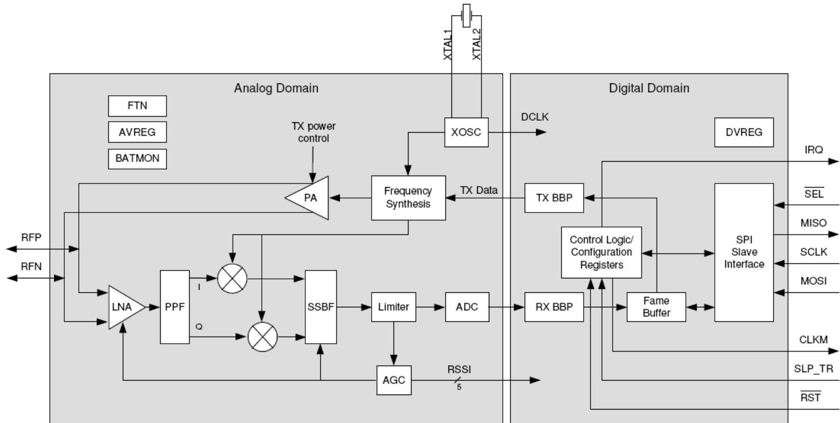
Figure 3-1. Block Diagram of the AT86RF230
