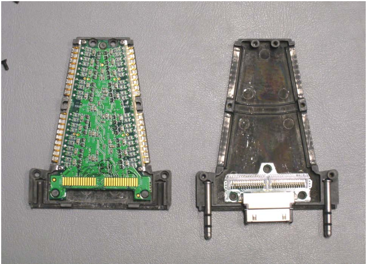
MOLE I/O Module, Internal, PCB internal sides
