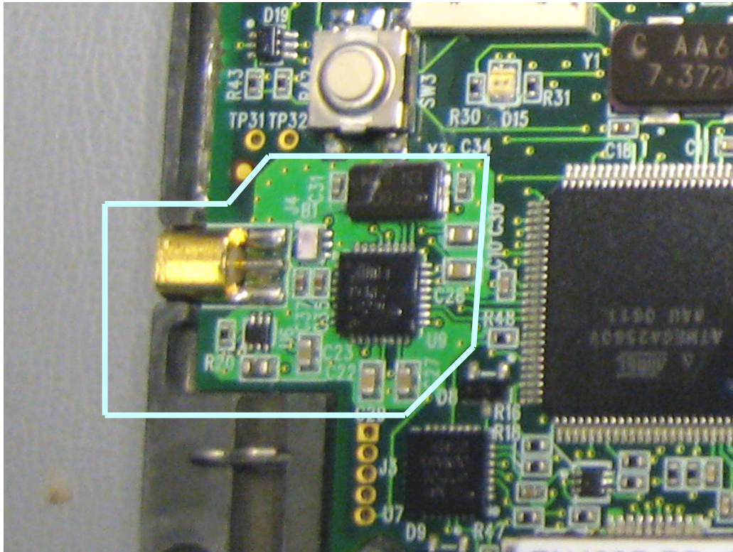
MOLE Main Module radio section
