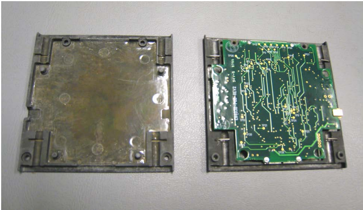
MOLE Main Module, Internal, PCB bottom
