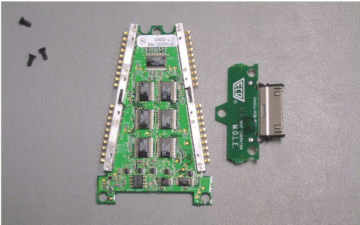
MOLE I/O Module, Internal, PCB external sides
