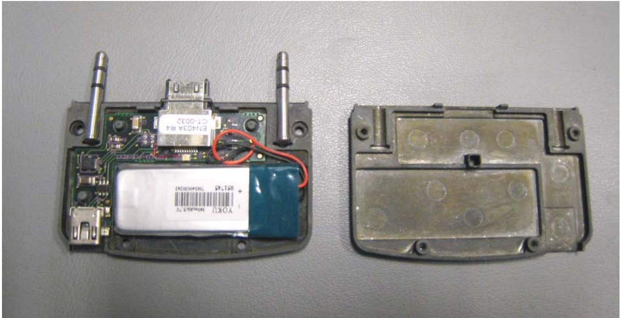
MOLE Battery Module, Internal, PCB top
