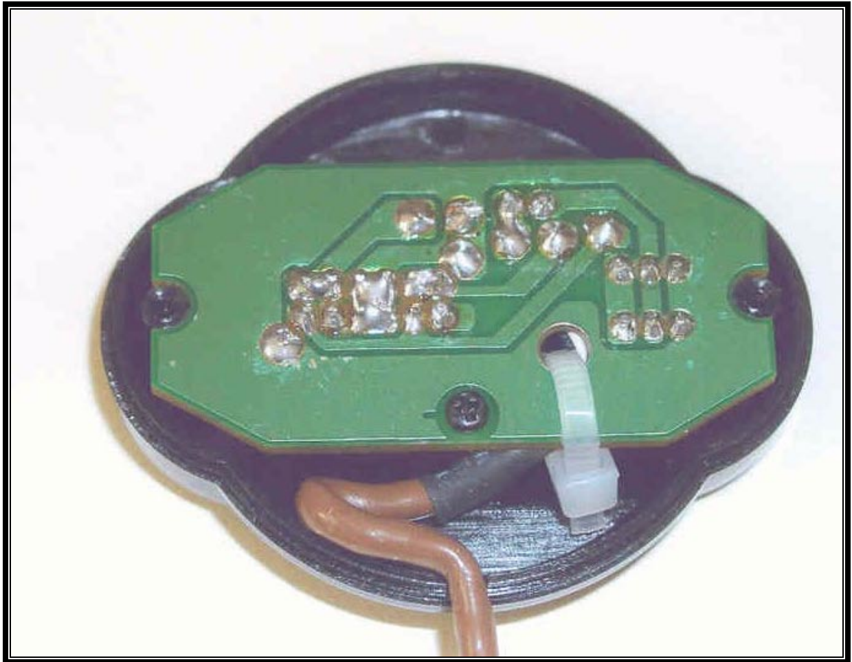
PHOTOGRAPH 11: SOLDER SIDE OF FM-10 Tx CONTROLLER PCB
