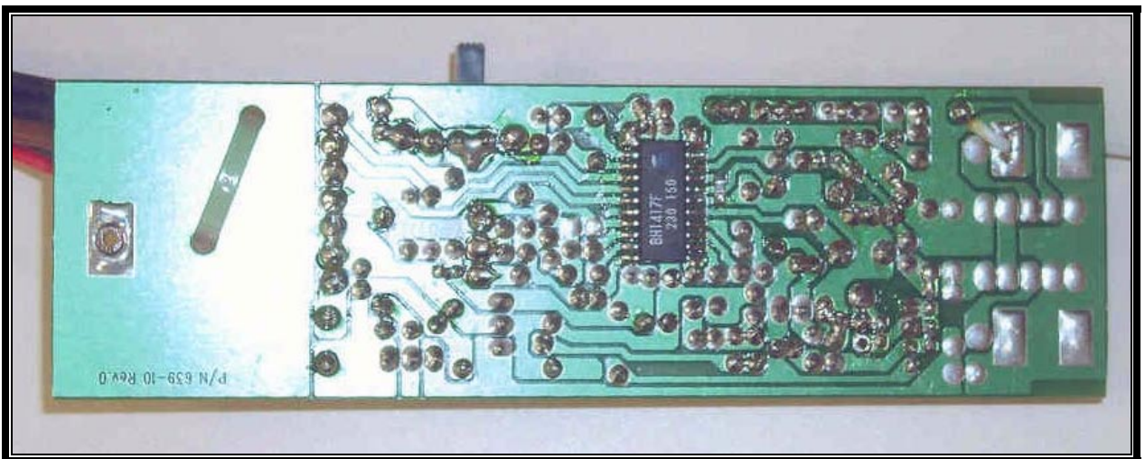
PHOTOGRAPH 9: SOLDER SIDE OF FM-10TX MAIN PCB
