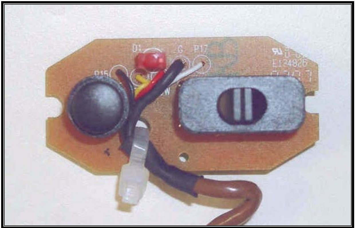
PHOTOGRAPH 10: COMPONENT SIDE OF FM-10 Tx CONTROLLER PCB
