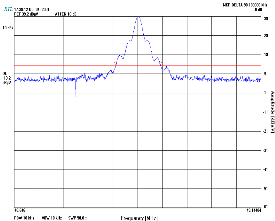
PLOT 6-1: OCCUPIED BANDWIDTH CHANNEL 1 (48.9 MHz)
