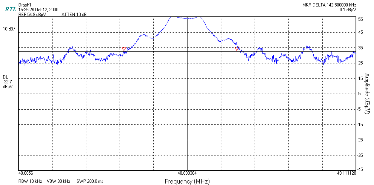
FIGURE 16: Channel 1 Occupied Bandwidth
