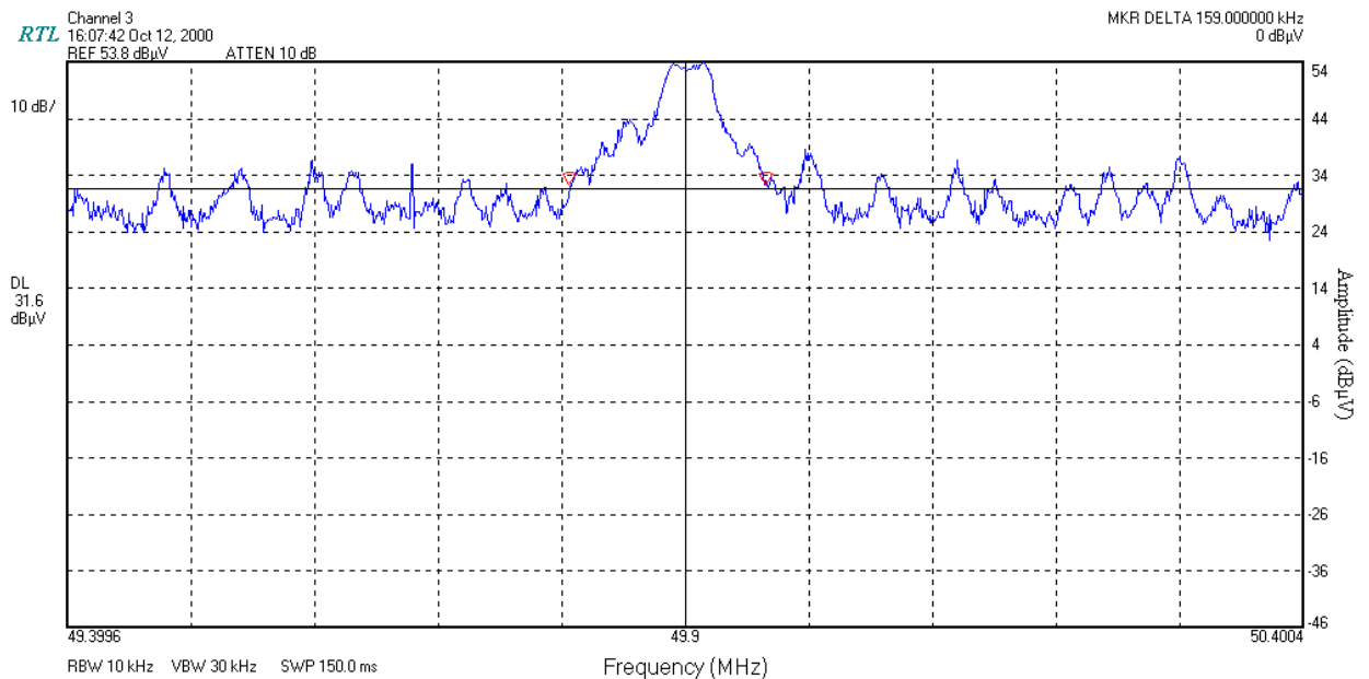
FIGURE 18: Channel 3 Occupied Bandwidth
