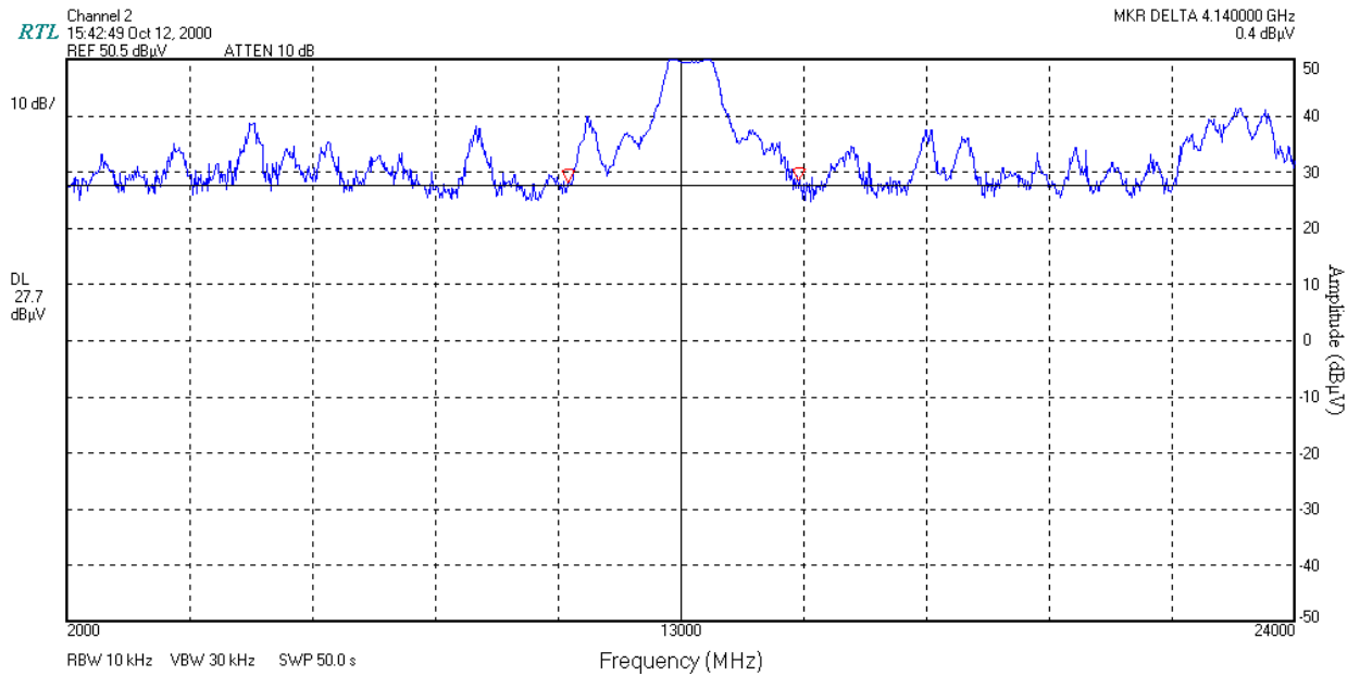
FIGURE 17: Channel 2 Occupied Bandwidth
