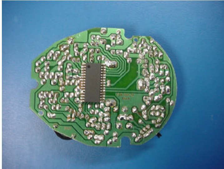
FIGURE 15: Headphone Right PCB Solder Side
