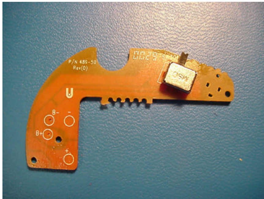
FIGURE 12: Headphone Left PCB Component Side
