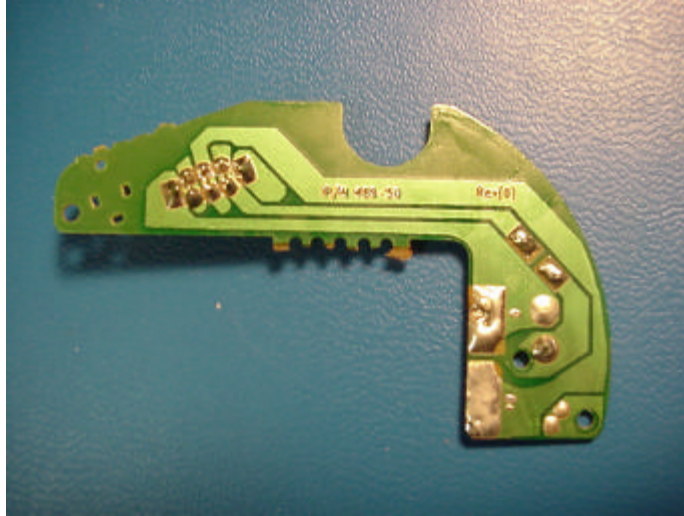
FIGURE 13: Headphone Left PCB Solder Side
