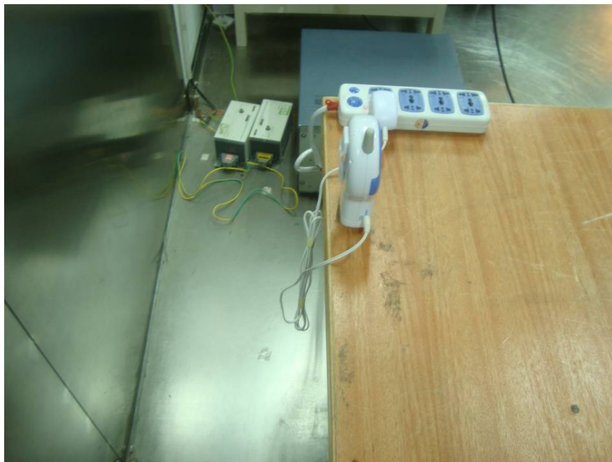
Charging mode: Conducted Emissions - Side View
