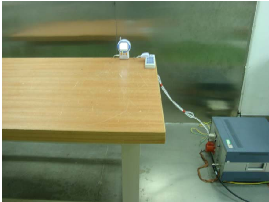
Transmitting mode: Conducted Emissions - Front View
