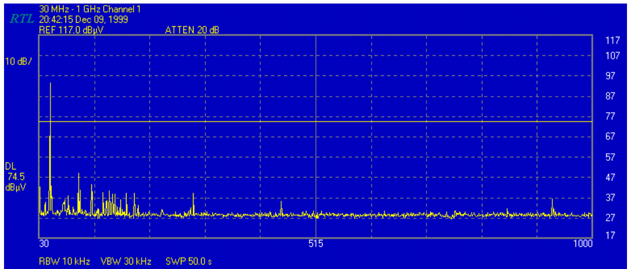
FIGURE 19: Channel 1 30 MHz – 1GHz Conducted
