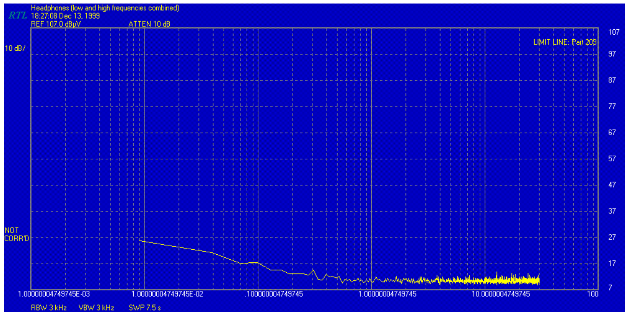
FIGURE 22: Receiver 9kHz – 30MHz (Low and High Frequency Combined)
