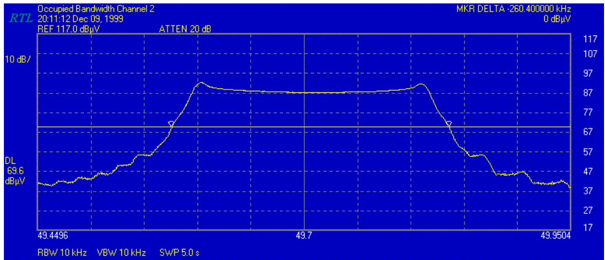
FIGURE 17: Channel 2 Occupied Bandwidth
