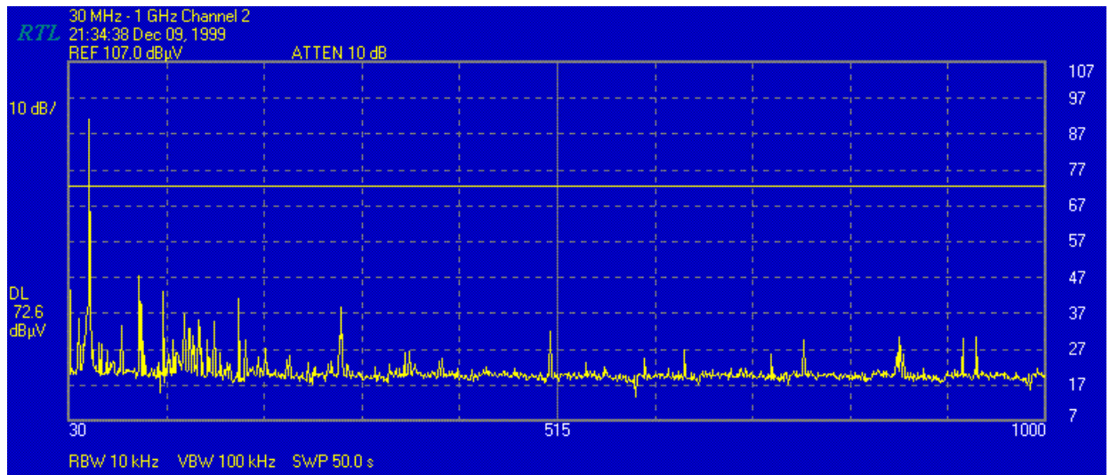
FIGURE 21: Channel 2 30MHz – 1GHz Conducted
