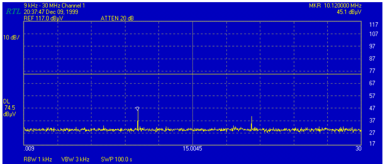
FIGURE 18: Transmitter Channel 1 9 kHz – 30 MHz Conducted
