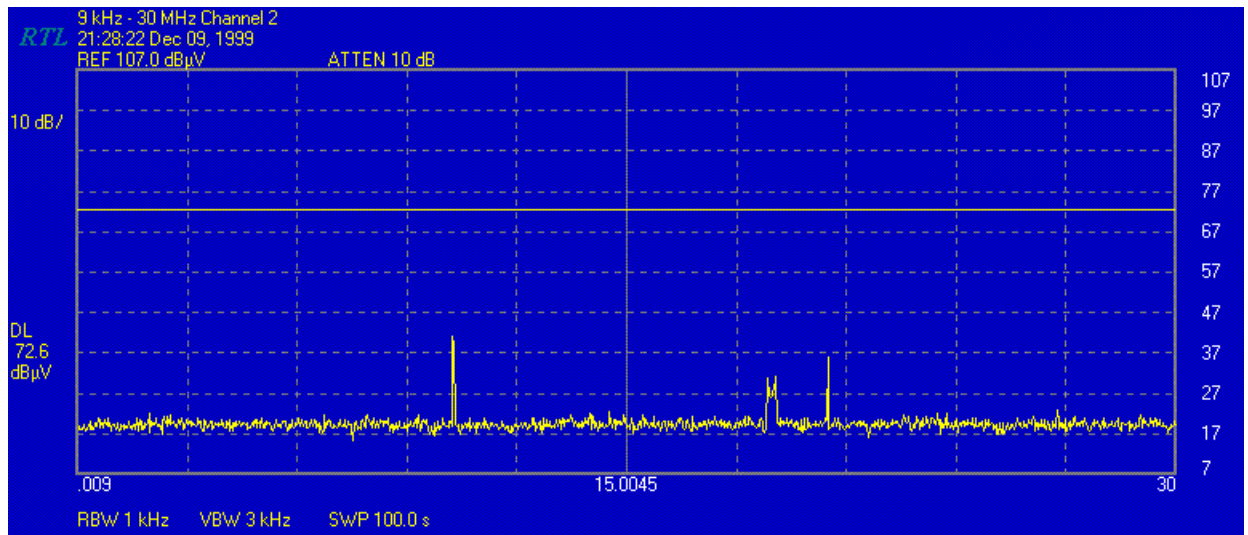
FIGURE 20: Channel 2 9kHz – 30MHz Conducted
