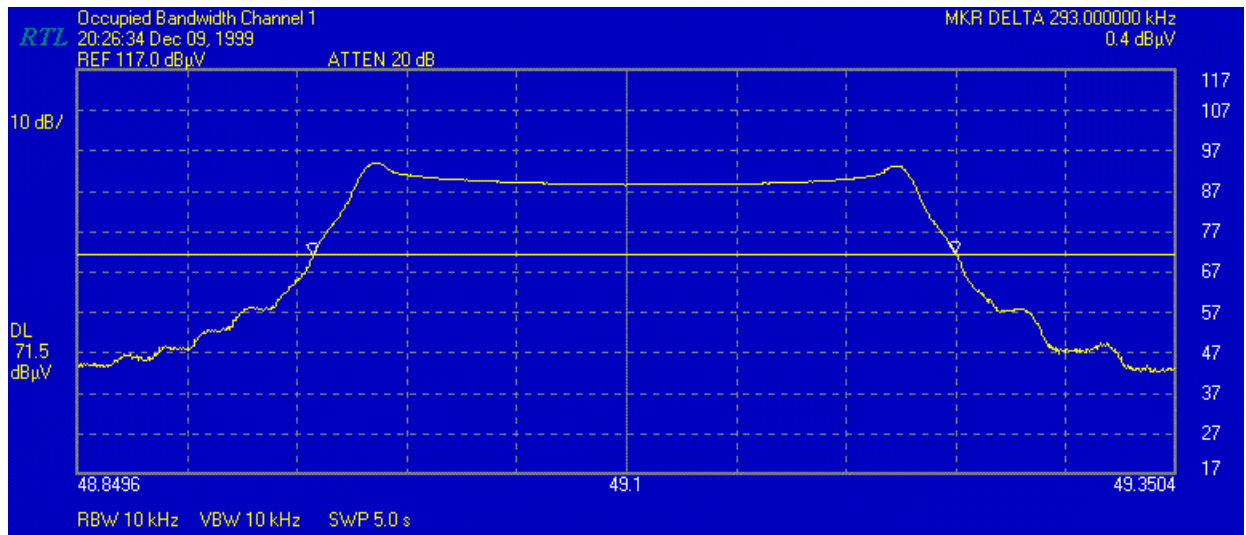
FIGURE 16: Channel 1 Occupied Bandwidth
