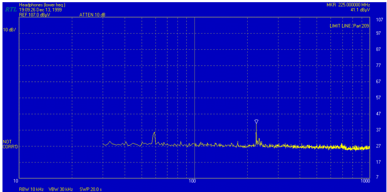
FIGURE 23: Receiver 30MHz – 1 GHz (Low Frequency) 48MHz
