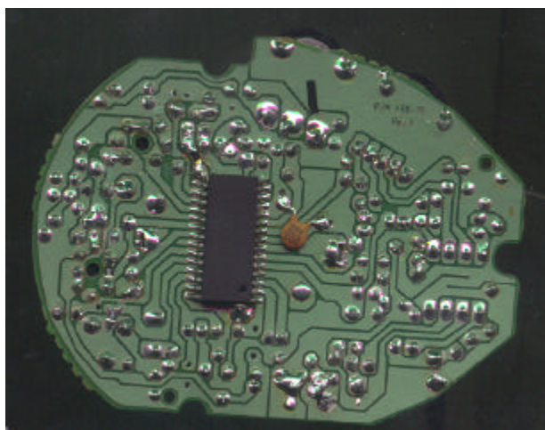
FIGURE 15: Headphone Right PCB Solder Side
