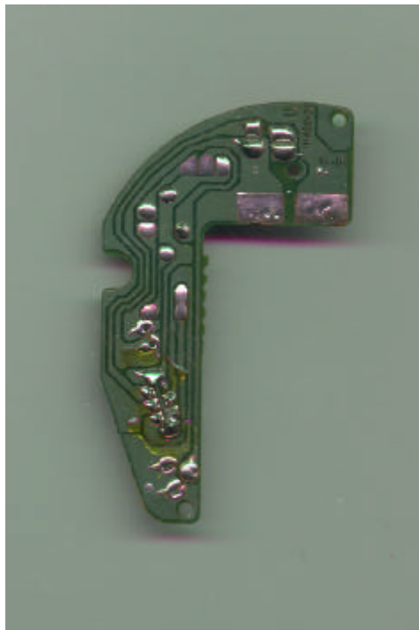
FIGURE 13: Headphone Left PCB Solder Side
