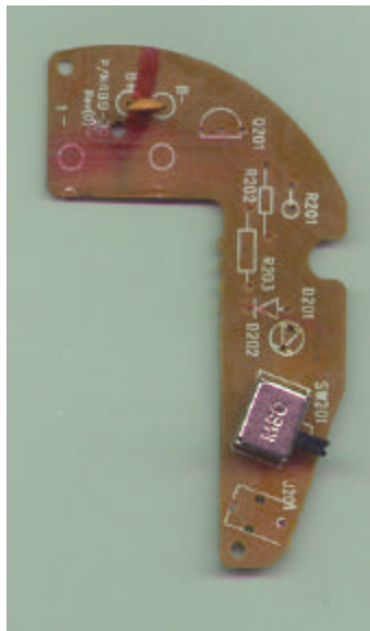
FIGURE 12: Headphone Left PCB Component Side
