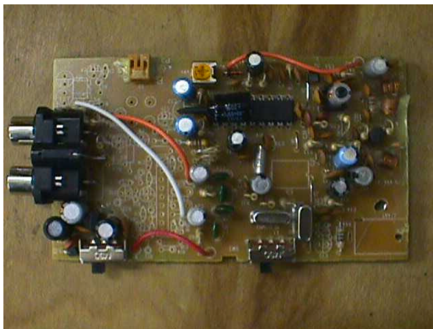
FIGURE 5: Transmitter Component Side
