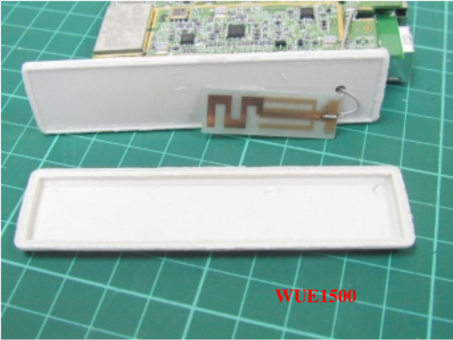
Photo 6: Inner view
