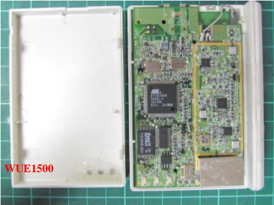
Photo 1: Inner view
