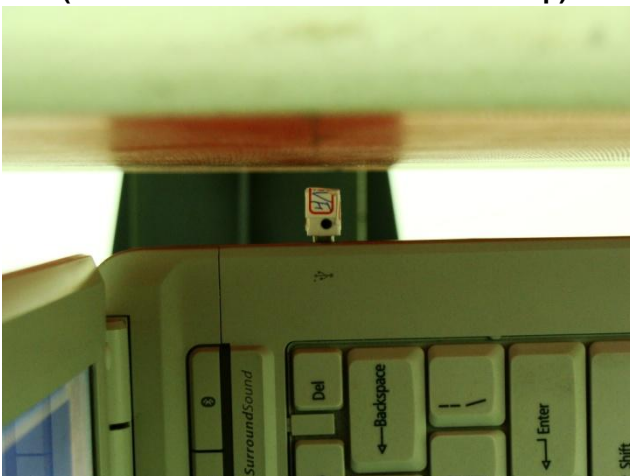
Direct Laptop Plug-in for USB Tip Mode (Tip of the DUT with Phantom 5 mm Gap)
