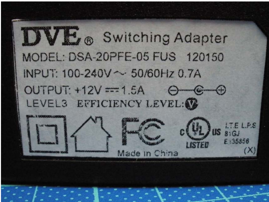
Adapter: DSA-20PFE-05 FUS 120150
