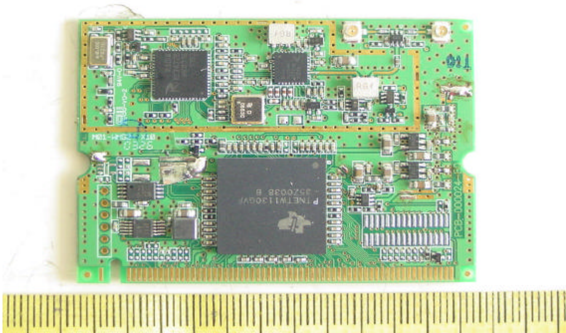
Solder View of Main PCB
