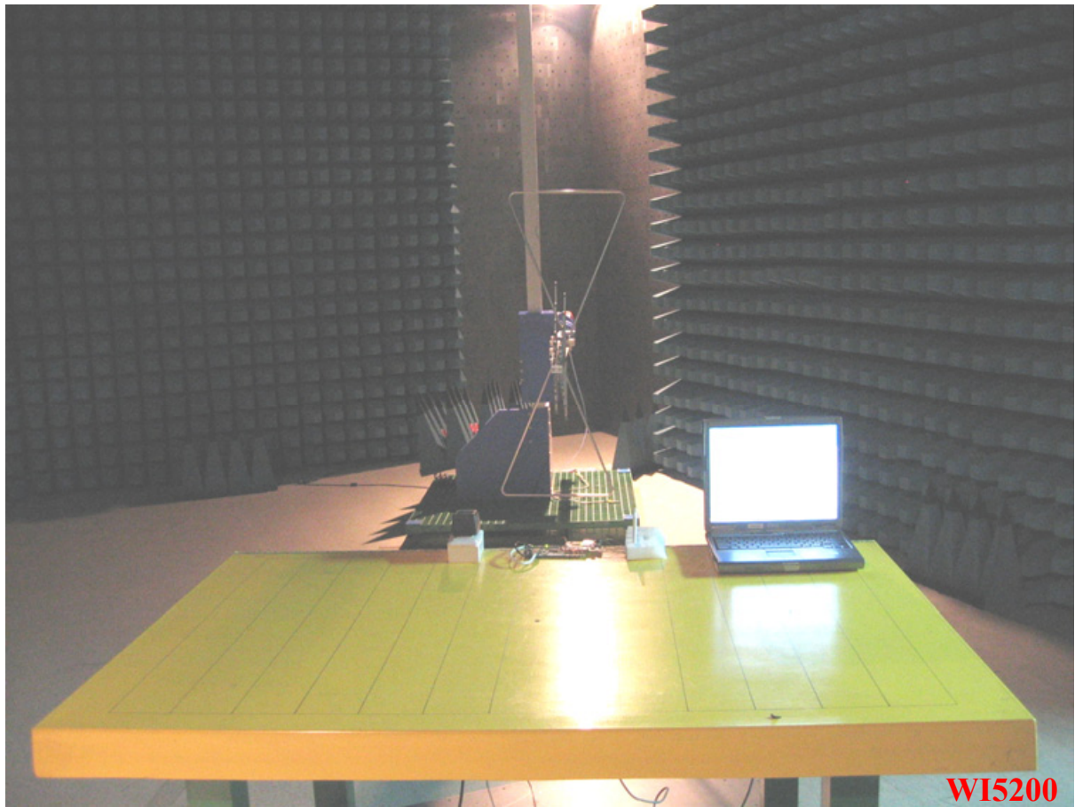
Photo 1: Radiated Emission Test set-up photo
