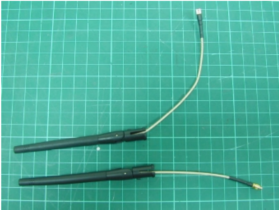
Photo 4: Antenna Photo (antenna A-1)
