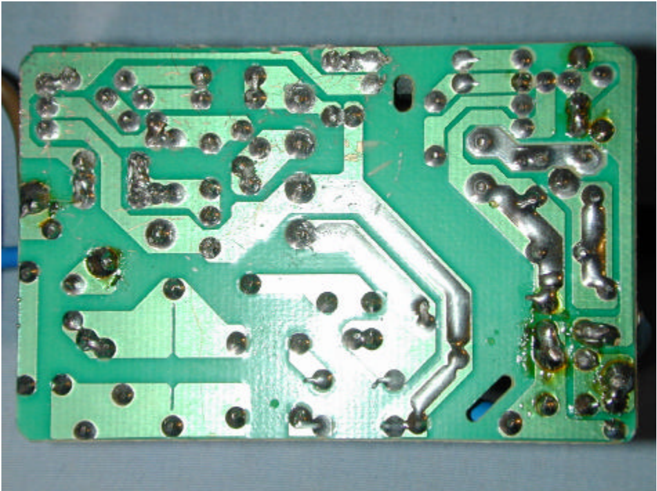
(11) EUT Photo
