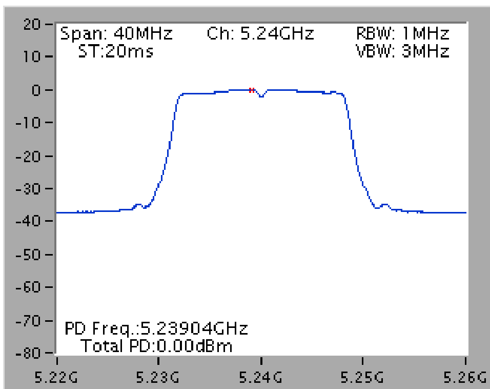
Power Density Plot on Configuration IEEE 802.11a / 5240 MHz
