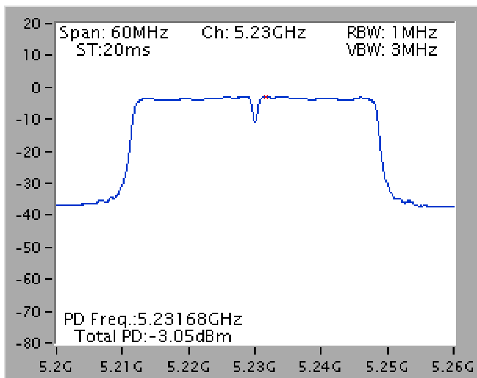
Power Density Plot on Configuration IEEE 802.11ac MCS0/Nss1 40MHz / 5230 MHz
