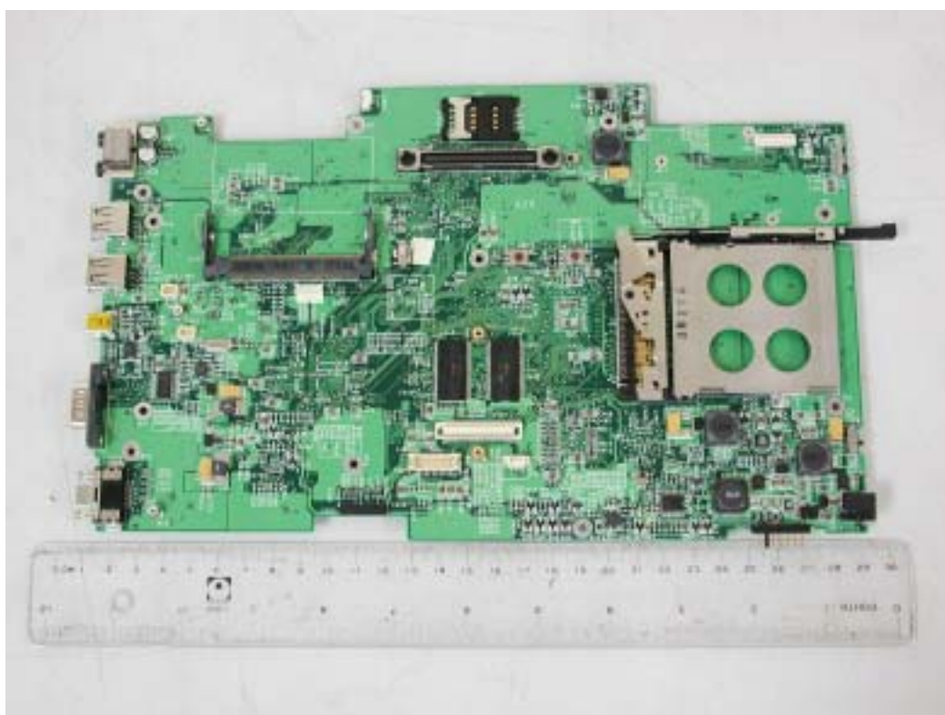
40. Front view of PCB6
