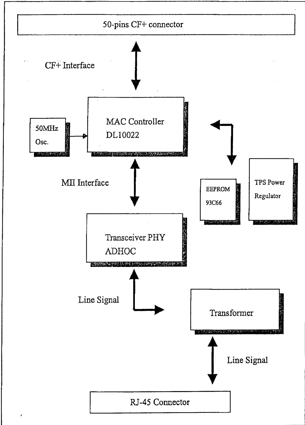
CompactFlash Size 10/100 Fast Ethernet LAN Card CFE100
