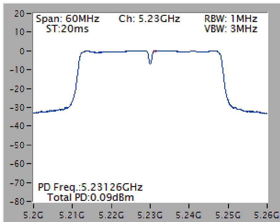
Power Density Plot on Configuration IEEE 802.11ac MCS0, Nss1 40MHz / Ant. 1 / 5230 MHz
