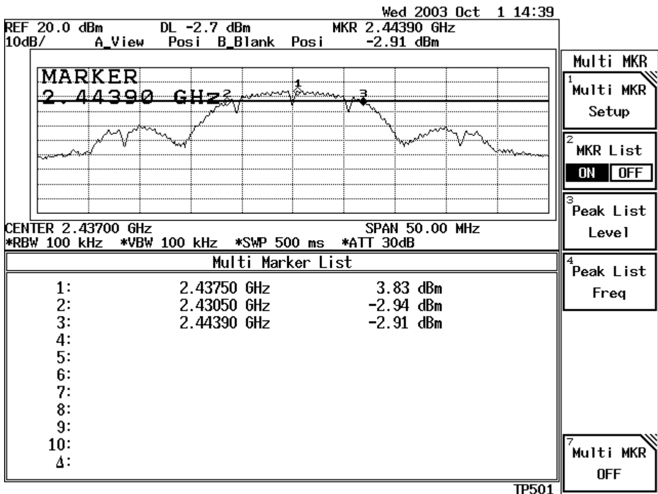
Figure Channel 6: 11Mbps
