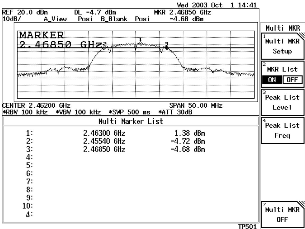
Figure Channel 11: 11Mbps
