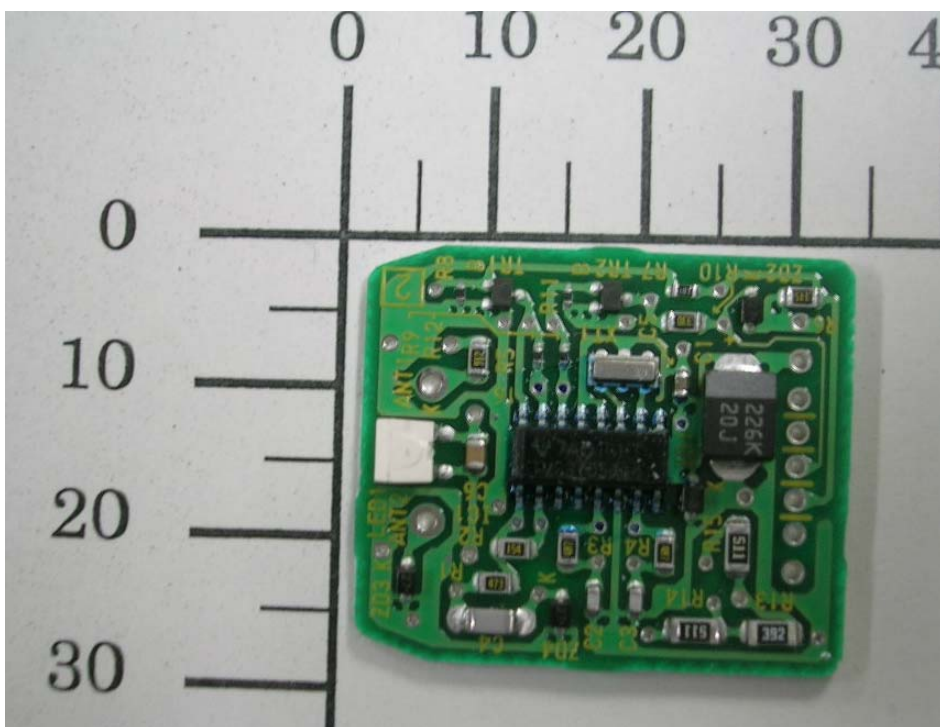
PC board (Reverse View)
