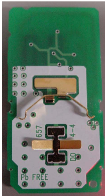
PC board (Reverse View)
