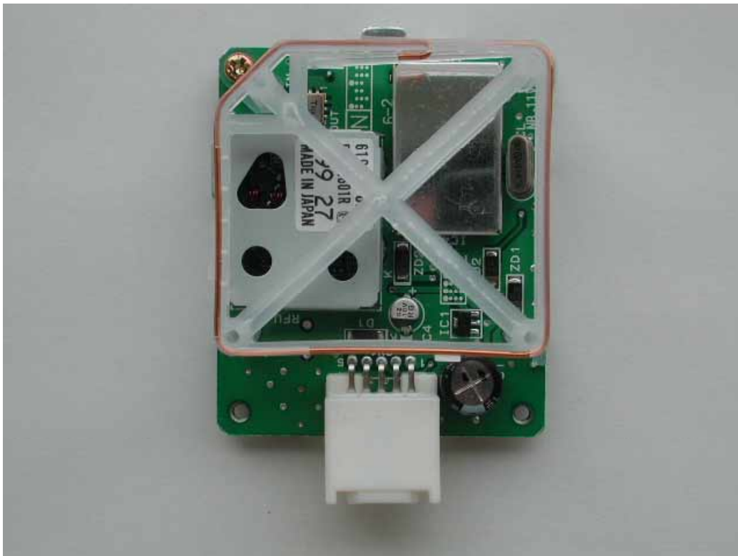
Mother PCB W/ Antenna PART No. D02PB
