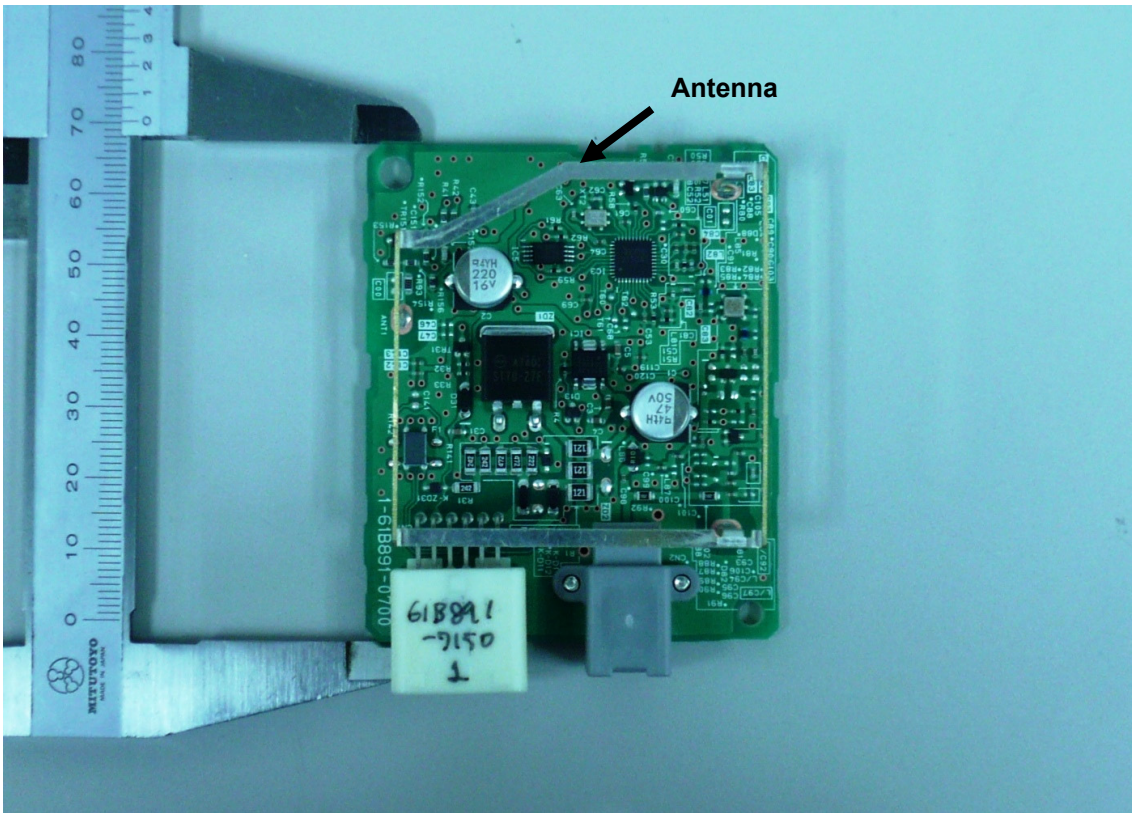
Top View(With Antenna)
