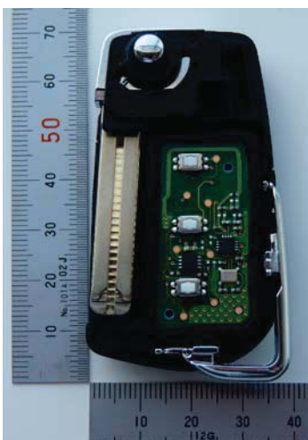
PC board inside the case
