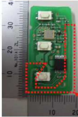
PC board (Front View)
