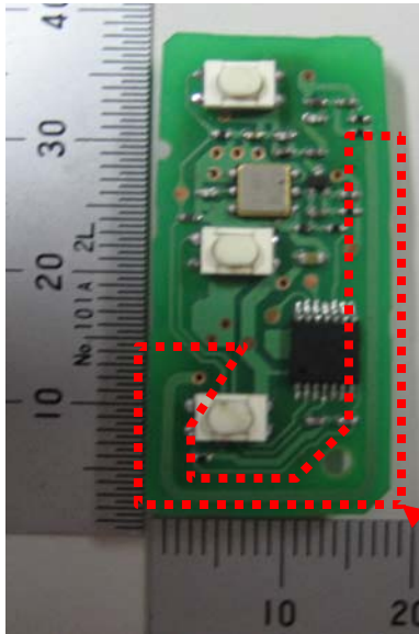
PC board (Front View)
