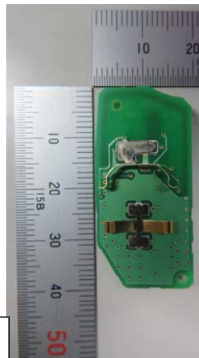
PC board (Rear View)
