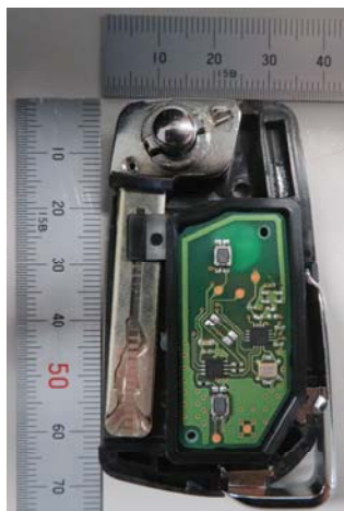
PC board inside the case
