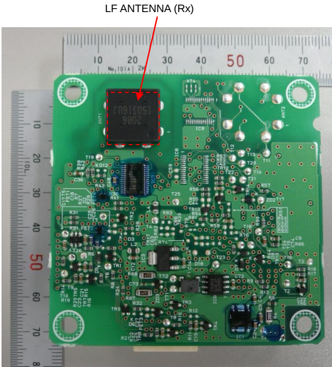
Reverse View
