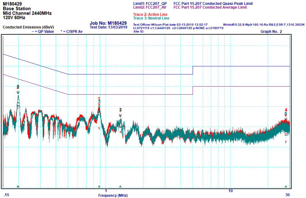
Graph 6-2: Conducted AC mains emission, 0.15 – 30 MHz, Middle channel – 2440 MHz
