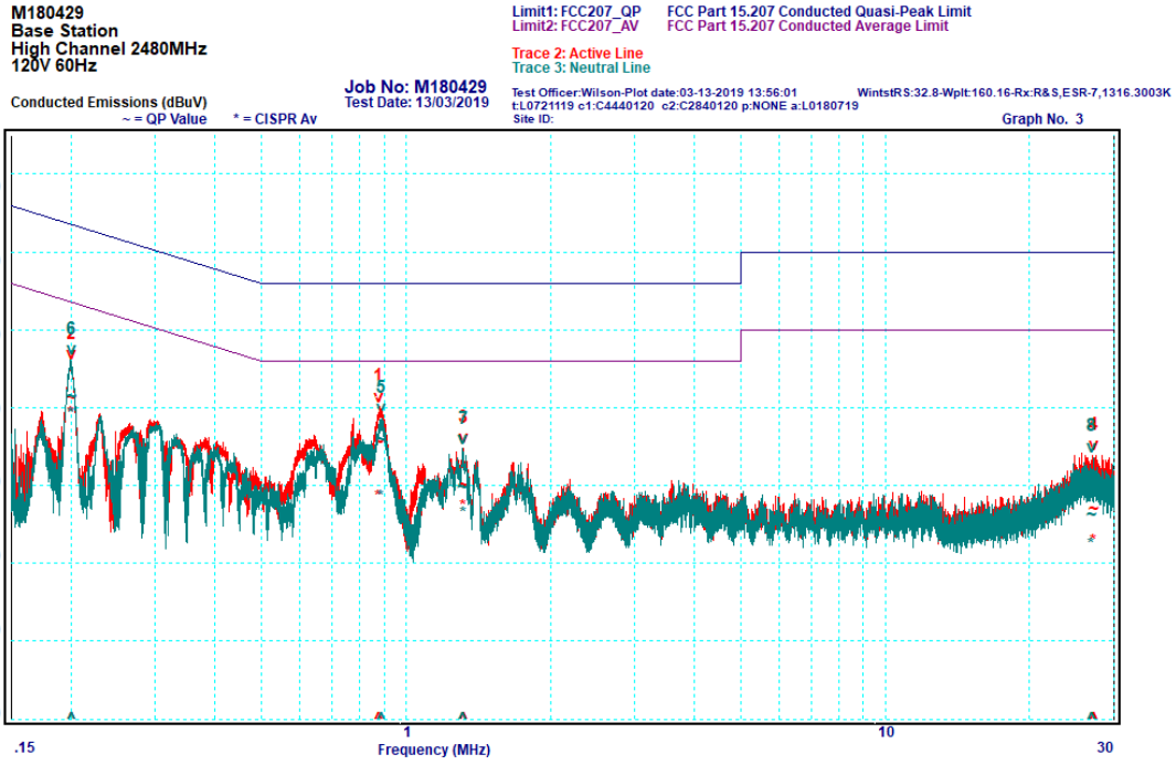
Graph 6-3: Conducted AC mains emission, 0.15 – 30 MHz, High channel – 2480 MHz
