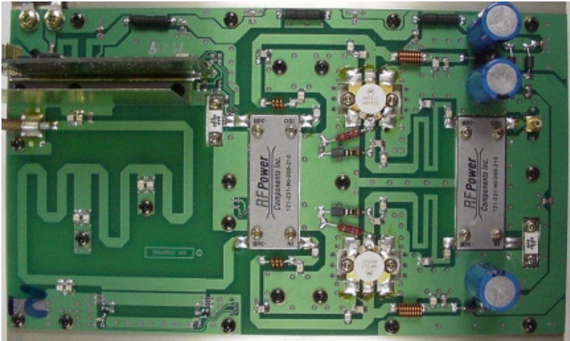
100 Watt Power Amplifier PC Board
