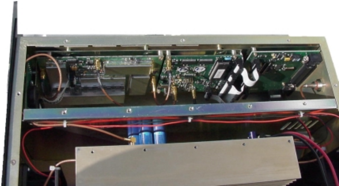
Digital and Modulation PCBs
