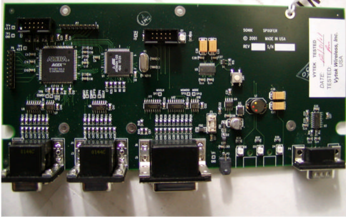
Power amplifier serial interface card (top view)
