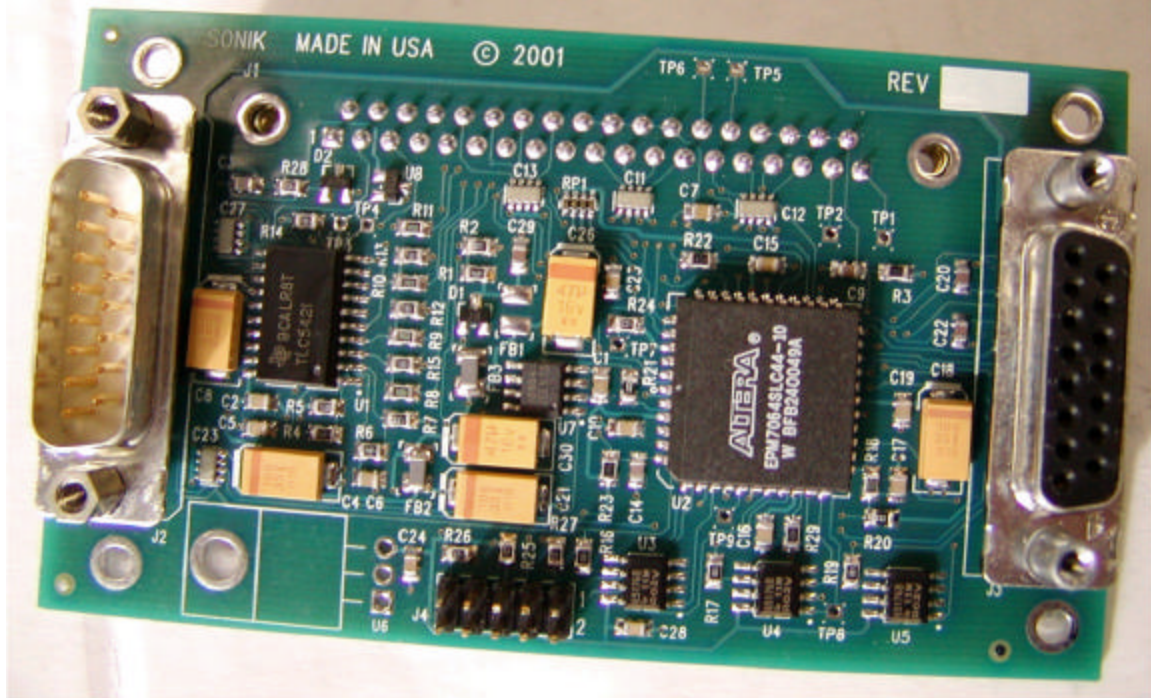
SPI CARD (top view)
