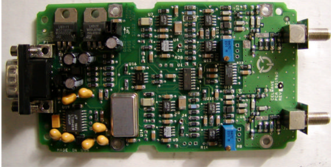
Internal wattmeter (top view)
