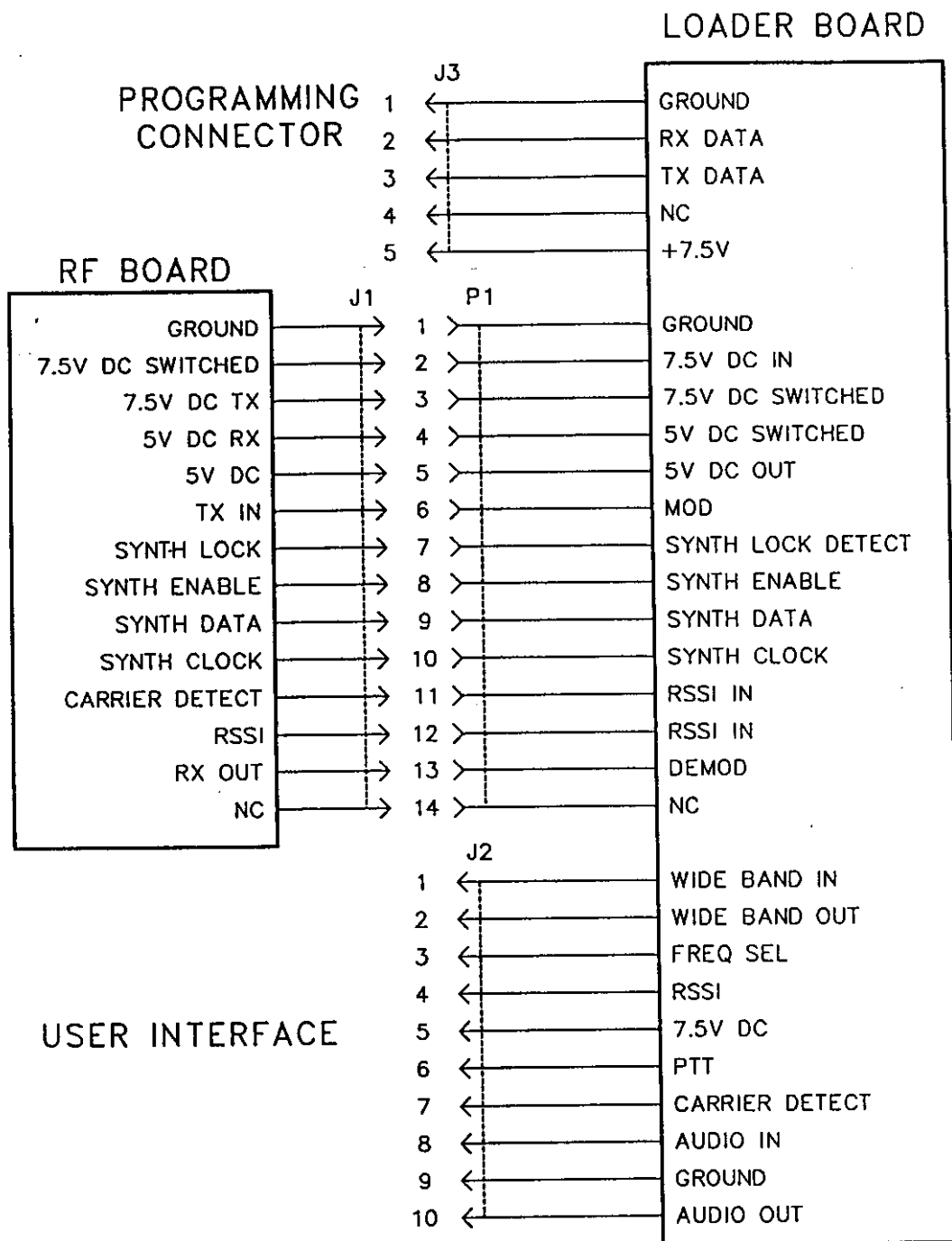
3472 INTERCONNECT SCHEMATIC (WITH LOADER BOARD) FIGURE 8-1
