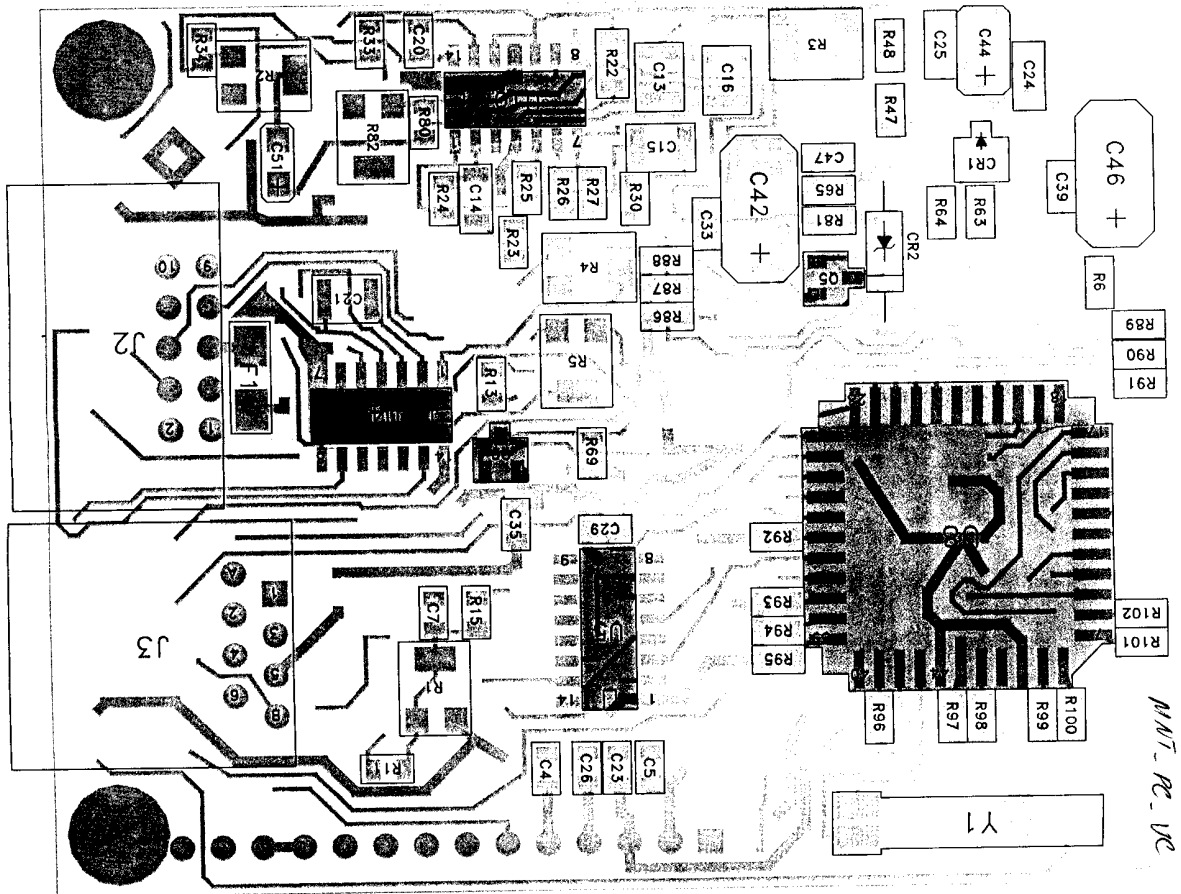
LOADER BOARD COMPONENT LAYOUT (TOP VIEW) FIGURE 8-9
