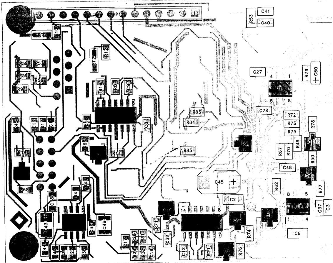
LOADER BOARD COMPONENT LAYOUT (BOTTOM VIEW) FIGURE 8-10
