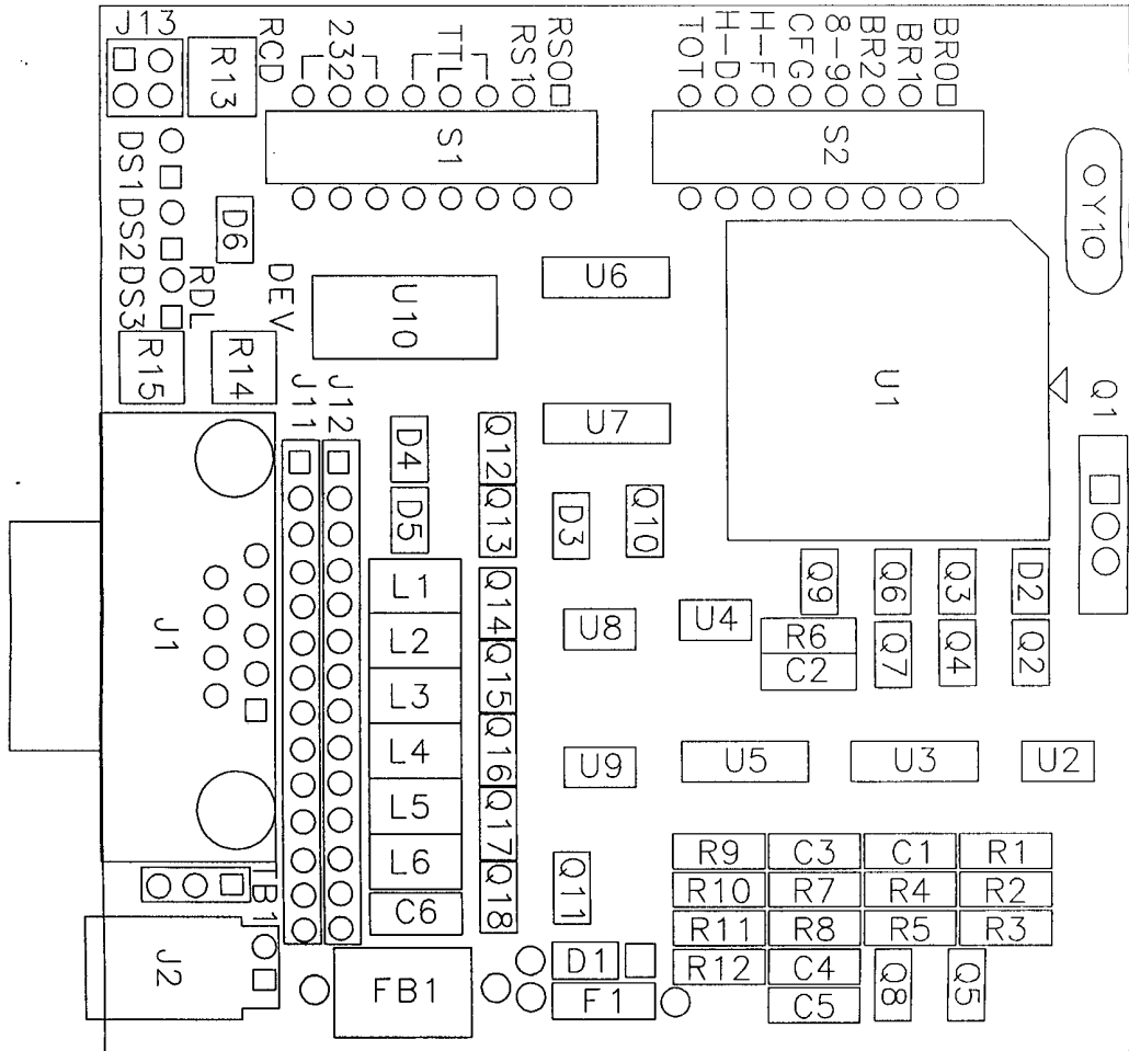
MODEM COMPONENT LAYOUT (COMPONENT SIDE) FIGURE 8-12
