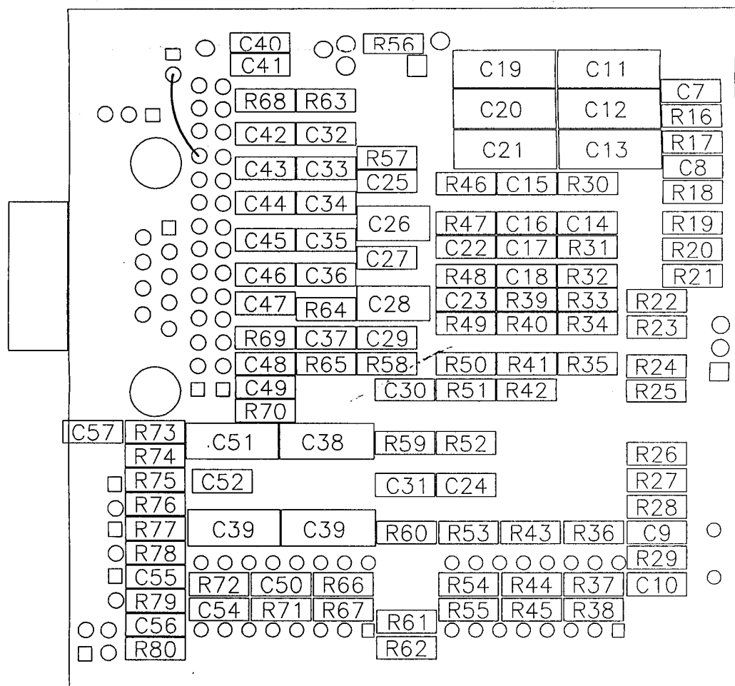
MODEM COMPONENT LAYOUT (SMD SIDE) FIGURE 8-13
